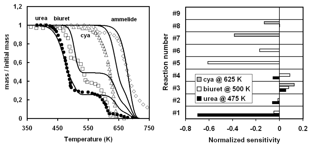
Figure 5: Cases 3 to 6 : a) Comparison of modeling results (lines) with experimental concentration profiles (symbols); b) Normalized sensitivity coefficients
