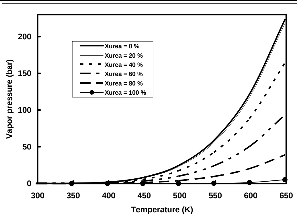
Figure 7: Vapor pressure diagram for urea-water solution at different temperatures and different mole fraction of urea in liquid phase.
