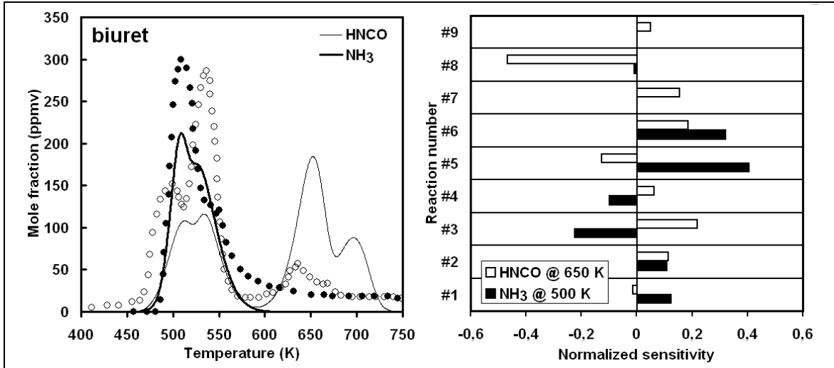
Figure 2: Case 2 : a) Comparison of modeling results (lines) with experimental concentration profiles (symbols); b) Normalized sensitivity coefficients
