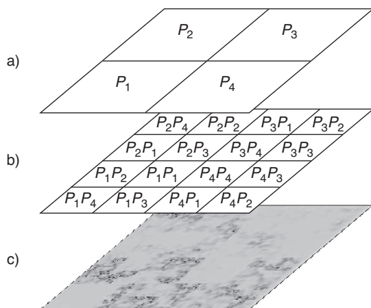
Figure 1 Multiplicative cascade algorithm.
