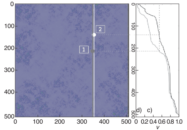
Figure 3 Differences between F_{x_1}^{-1}(u) and F_{x_2}^{-1}(u) when x changes from x_1 to x_2 yielding a jump in the vertical direction.
