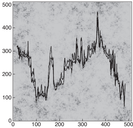
Figure 2 Discontinuous gradual deformation trajectory of a single point using the sequential method.
