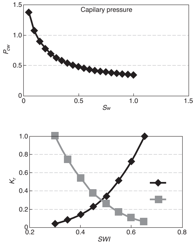
Figure 6 Capillary pressures and relative permeabilities for the initial model.
