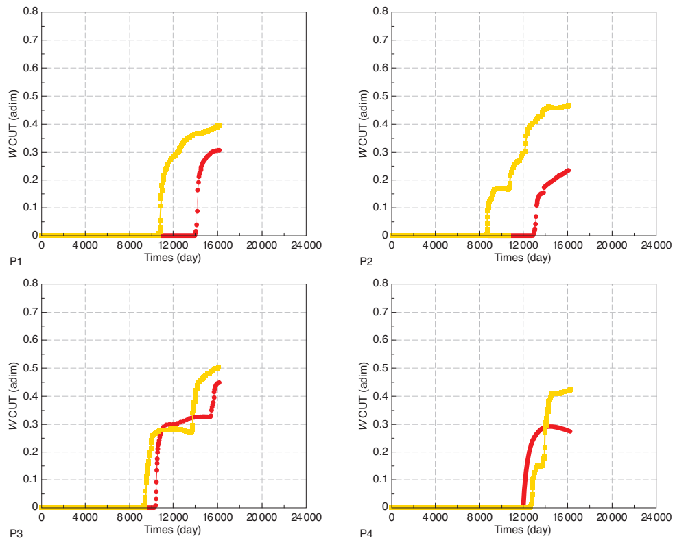
Figure 12 Initial water cut levels for P1, P2, P3 and P4. Field production data is in red, and simulated values in yellow.
