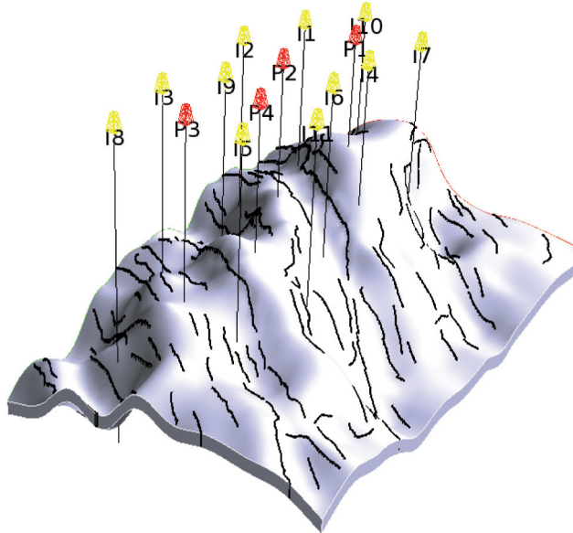
Figure 7 Bloemendaal reservoir structure: 11 injection wells and 4 production wells. Seismic faults are represented in black.
