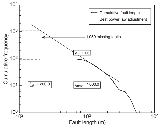
Figure 8 Extension of the power law. The model choice “ l_{min} = 200 m” provides the number of subseismic faults to generate.
