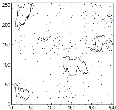
Figure 5 Deformation trajectories with the multiscale sequential method.
