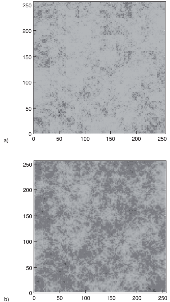
Figure 4 Non interpolated a) and interpolated b) multiplicative cascades.
