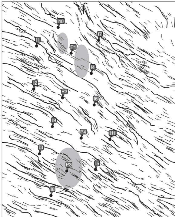
Seismic fault (black lines), initial sub-seismic fault realization (gray lines) and elliptic study zones (gray).
