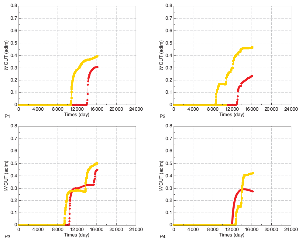
Initial water cut levels for P1, P2, P3 and P4. Field production data is in red, and simulated values in yellow.
