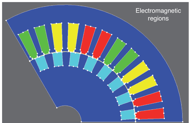
Figure 14 Representation of an asynchronous motor in Flux2D.
