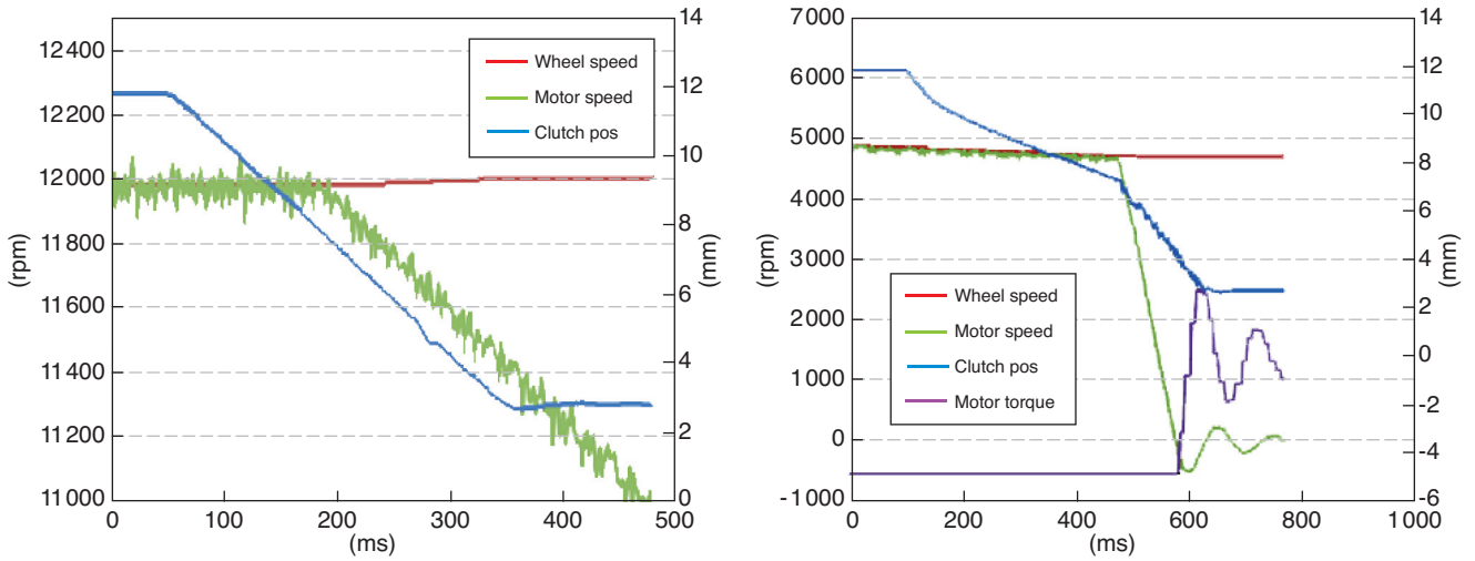
Figure 6 Clutch disengagement under nominal condition without torque at 85 km/h (up) and under 5 Nm torque (down).
