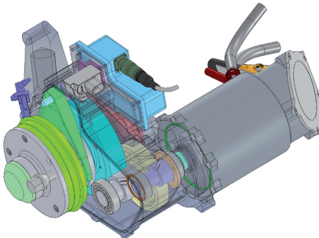
Figure 7 In-wheel motor and clutch integration.
