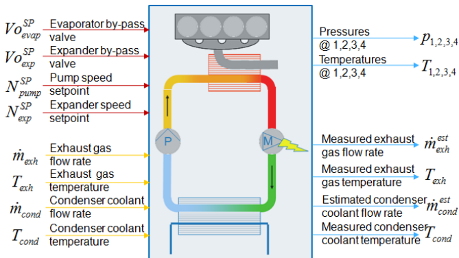
Fig. 2. Rankine steam process IO
