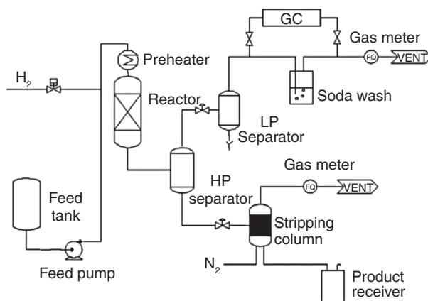
Figure 2 Flow scheme of the pilot plant.
