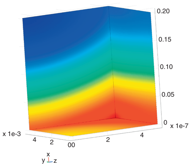
Figure 8 Adsorbed oxygen at the crystallite scale.
