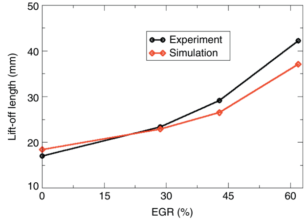
Figure 10 Evolution of the LOL as a function of the EGR rate.
