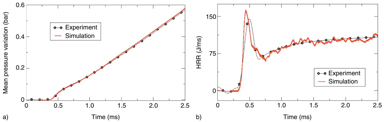
Figure 5 Temporal evolution of the mean pressure variation a) and the HRR b) for the 0% EGR experiment and simulation.
