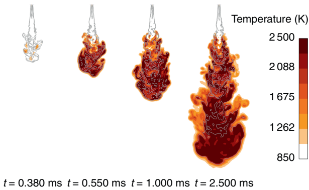
Figure 6 Temperature fields at four different times after SOI for the configuration with 0% EGR. The grey lines represent equivalence ratio isolines at 0.5, 1 and 2.
