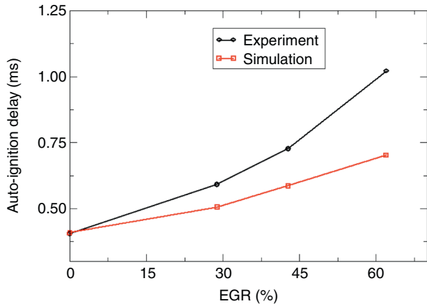
Figure 9 Auto-ignition delay as a function of the EGR rate.
