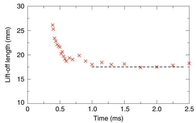
Figure 7 Temporal evolution of the LOL for the LES of the 0% EGR case. The dashed line represents the experimental stabilised LOL value.
