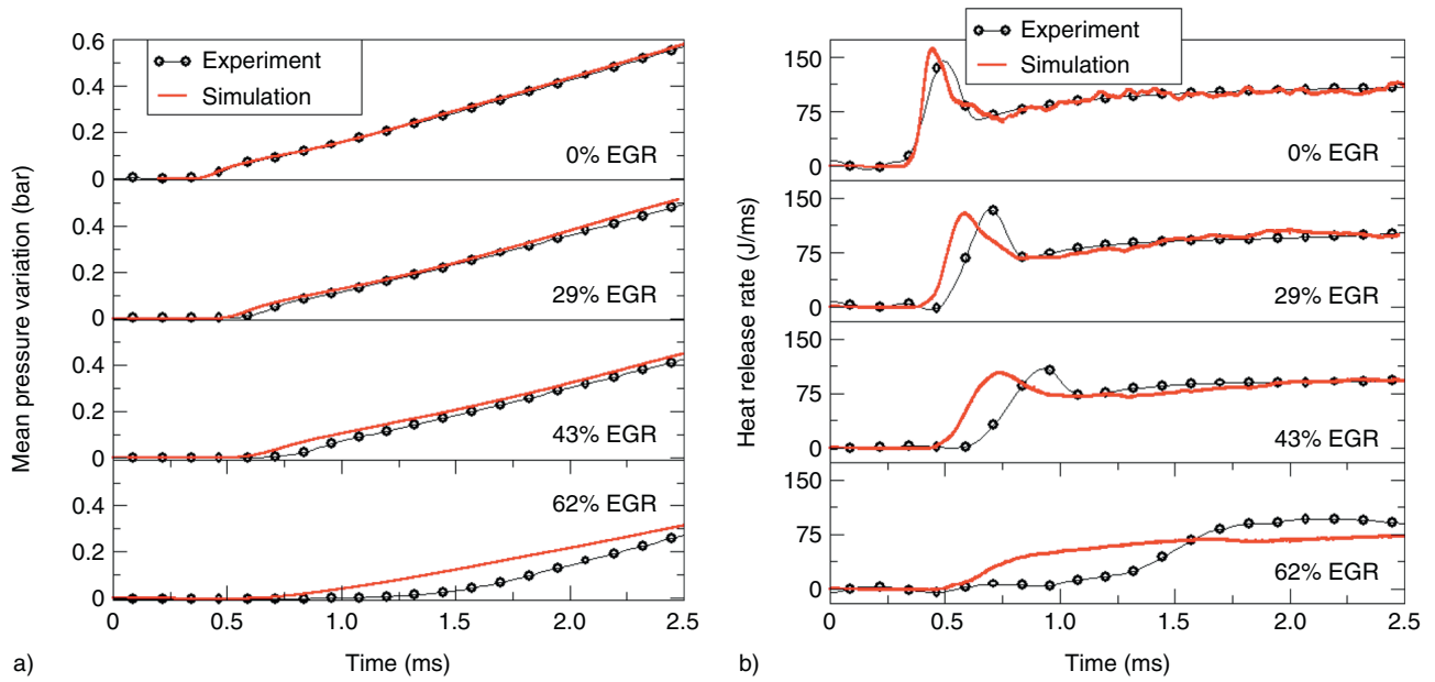
Figure 8 Temporal evolution of a) the mean chamber pressure and b) the HRR in the experiment and simulation for the four EGR rates.
