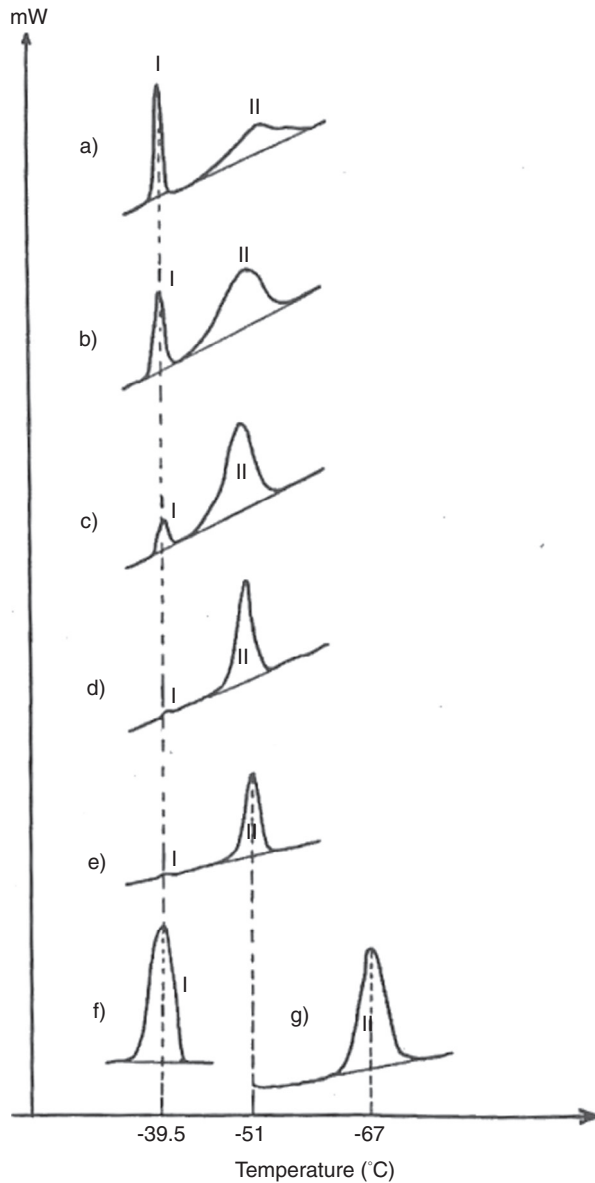
Figure 10 DSC cooling curves of W/O mixed emulsion with pure water droplets and water + NaCl droplets dispersed in oil media at successive time intervals a) t = 2 min; b) t = 25 min; c) t = 43 min; d) t = 62 min; e) t = 82 min after the mixing of f) emulsion 1 (pure water and g) emulsion 2 (water + NaCl) (from [49]).
