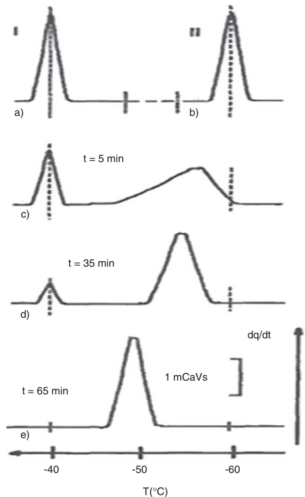
Figure 7 DSC cooling curves of W/O mixed emulsion with pure water droplets a) and water + urea droplets b) dispersed in oil media at successive time intervals c) t = 5 min; d) t = 35 min; e) t = 65 min, exothermic signal upwards (from [48]).
