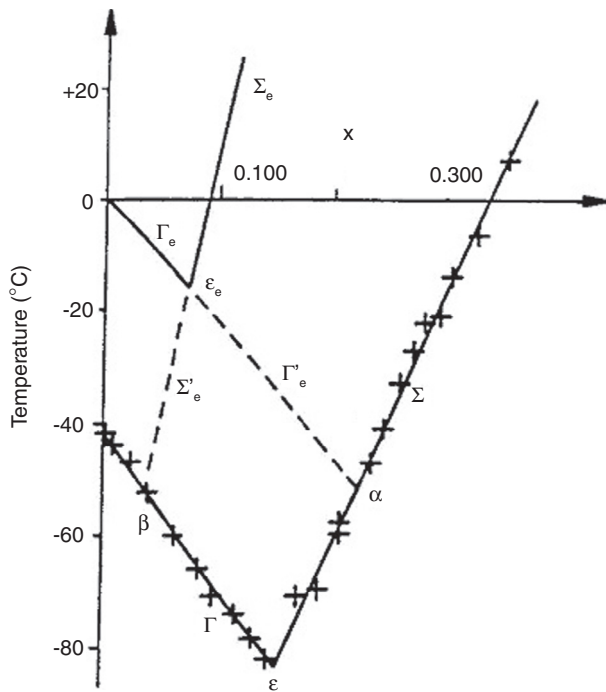
Figure 6 Freezing curves for the binary \text{NH}_4\text{Cl} + \text{H}_2\text{O} dispersed within a W/O emulsion.
