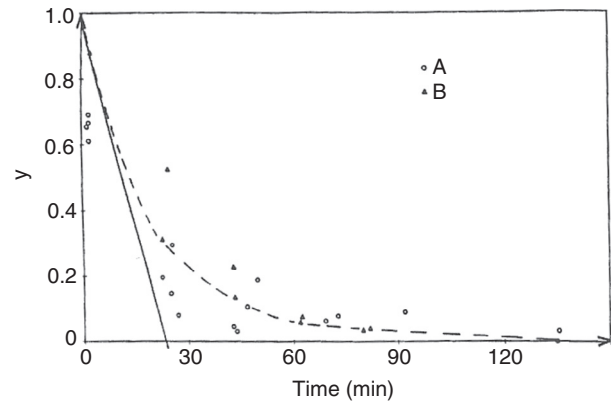
Figure 11 Percentage \gamma of pure water moles numbers transferred in W/O mixed emulsion with pure water droplets and water + NaCl droplets dispersed in oil media (oil A or oil B), versus time (from [49]).
