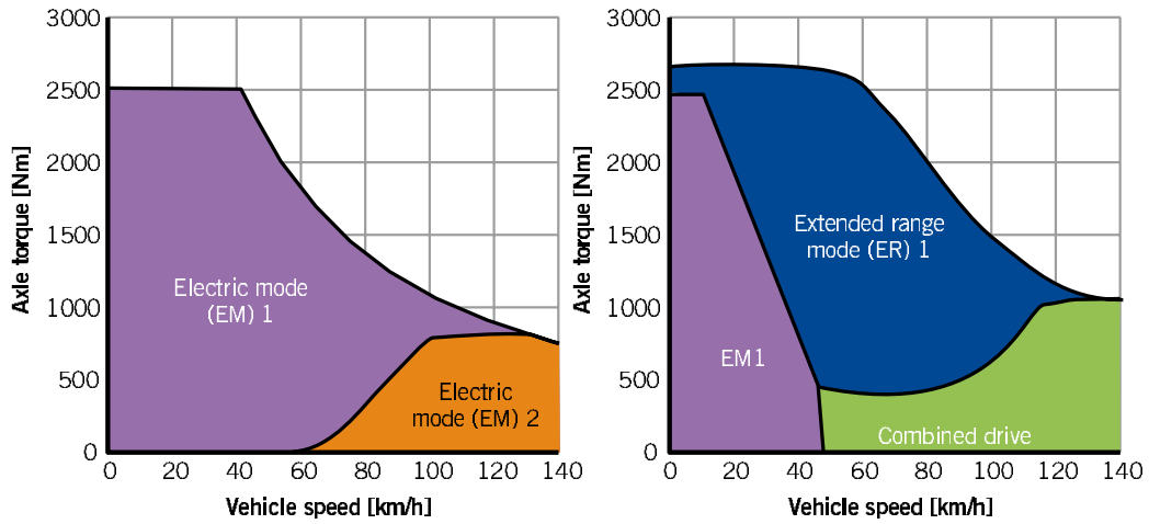
Figure 7: Operating modes of GM's Volt as a function of vehicle speed and desired torque [33].
