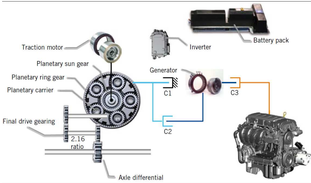
Figure 2: Kinematic architecture of GM's Volt [33].
