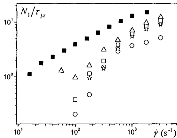
22 23 24 25 26 27 28 29 30 31 32 33 34 35 36 37 38 39 40 41 42 43 44 45 46 47 48 49 50 51 52 53 54 55 56 57 58 59 60 61 62 63 64 65 Figure 15: Ratio of the normal to the shear stress as a function of the shear rate for PAM6000 (filled squares) and for PEGPEO at different concentrations: (circles) 500, (stars) 1500, (open squares) 2000, (triangles) 3000 ppm.
