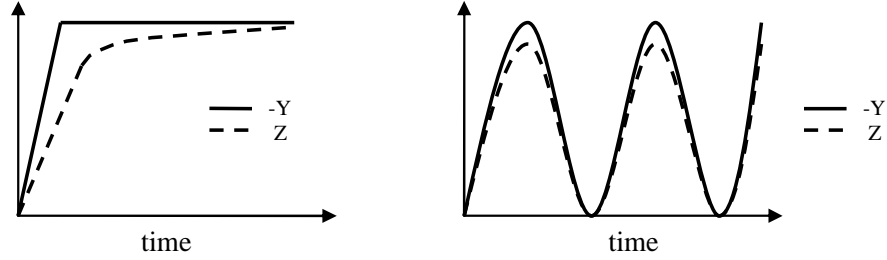
Fig. 1 Role of Z in creep and fatigue modeling
