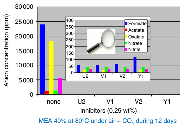
Figure 9 Concentration of HSS in solvent using different inhibitors.
