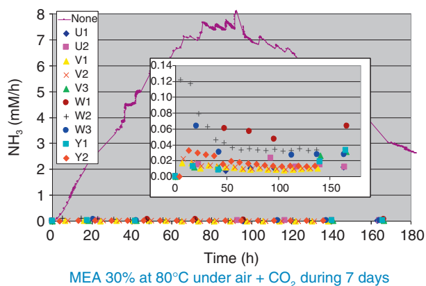
Figure 10 Concentration of NH 3 in the outlet gas for different inhibitors.
