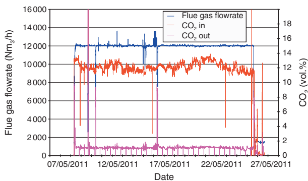
Figure 15 Parameters trend for MEA 40 wt% – long run test.
