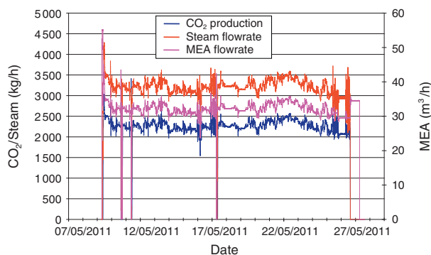
Figure 14 Parameters trend for MEA 40 wt% – long run test.
