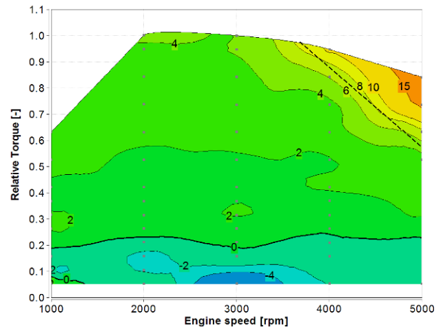
Figure 19: BSFC gap between CR 10.5 and CR 12 (from green to orange \Rightarrow BSFC 12 < BSFC 10.5, dashed line denotes the fuel enrichment limit at CR 10.5)
