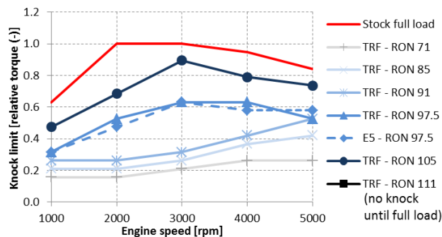
Figure 3: Knock limit for different RON at CR 10.5:1
