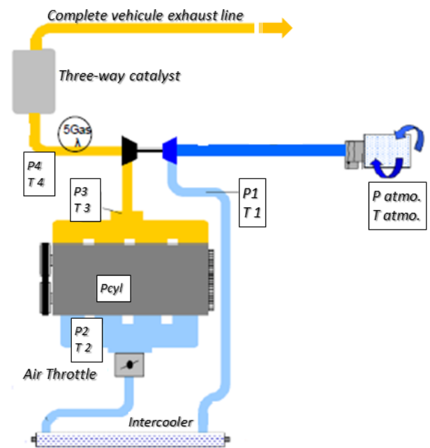
Figure 2: Equipped engine at test bench
