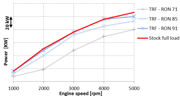
Figure 6: Full load curve for different RON at CR 10.5:1 expressed in effective power (limits: CA50 = 30°CA or FAER = 1.3)
