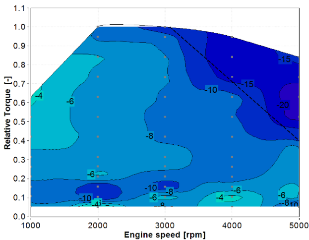
Figure 18: BSFC gap between CR 7.5 and CR 10.5 (blue \Rightarrow BSFC 10.5 < BSFC 7.5, dashed line denotes the enrichment limit at CR 7.5)
