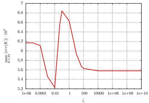
Figure 14: Maximum of model error as a function of \zeta .
