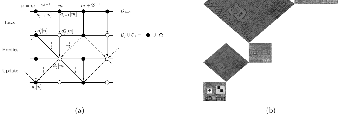
Figure 28: (a) Predict and update lifting steps (b) MaxMin lifting of the Haar-Riesz Memorial plaque.
