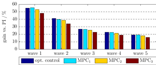
Fig. 16. Performance gain (with respect to the PI control) of the optimal control, an MPC with state feedback and perfect wave prediction (MPC 1 ), an MPC with output feedback and perfect wave prediction (MPC 2 ) and an MPC with output feedback and AR identification based wave prediction (MPC 3 ). Only the representative time interval [301 sec, 501 sec] is considered.
