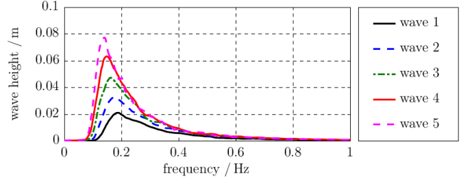
Fig. 3. The (smoothed) spectra of the five considered sea states.
