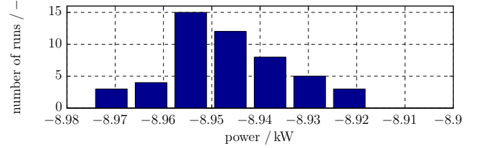
Fig. 6. Distribution of average power harvested with optimal controls calculated using random initial values.
