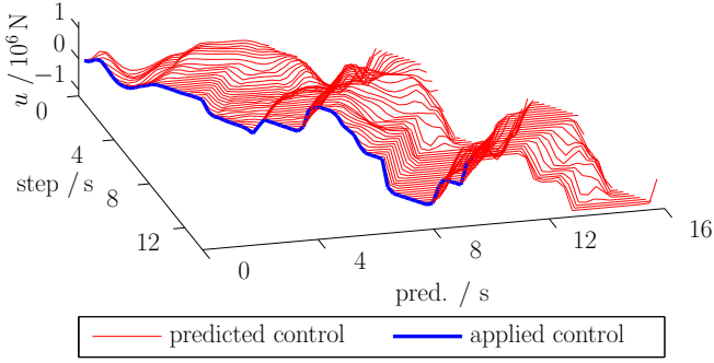
Fig. 11. Applied and predicted controls in a sliding horizon MPC scheme. The red lines represent u_{c,i} in each time step. The first entry, i.e. the applied control, is highlighted in blue.
