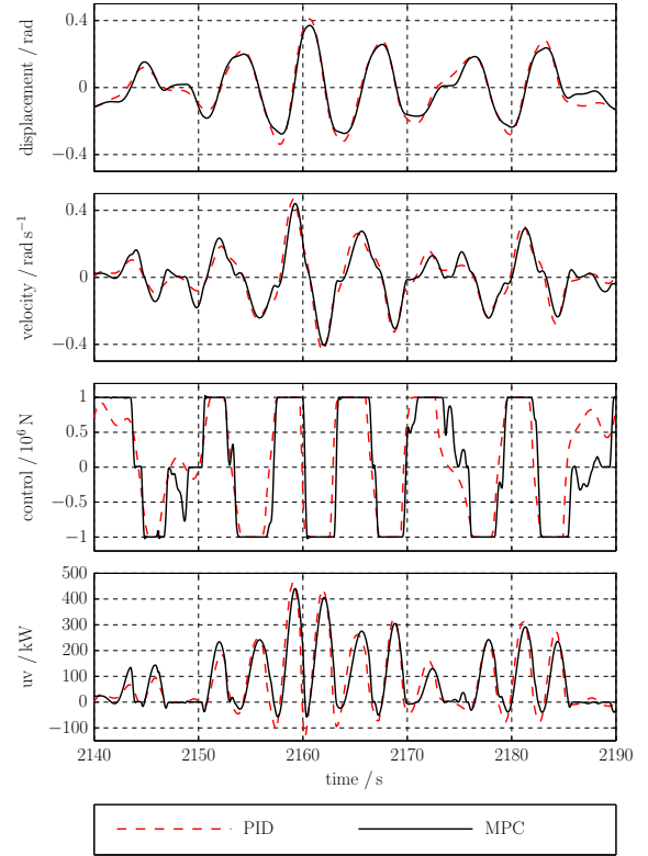
Fig. 15. Comparison of MPC and PI control for the wave 5.
