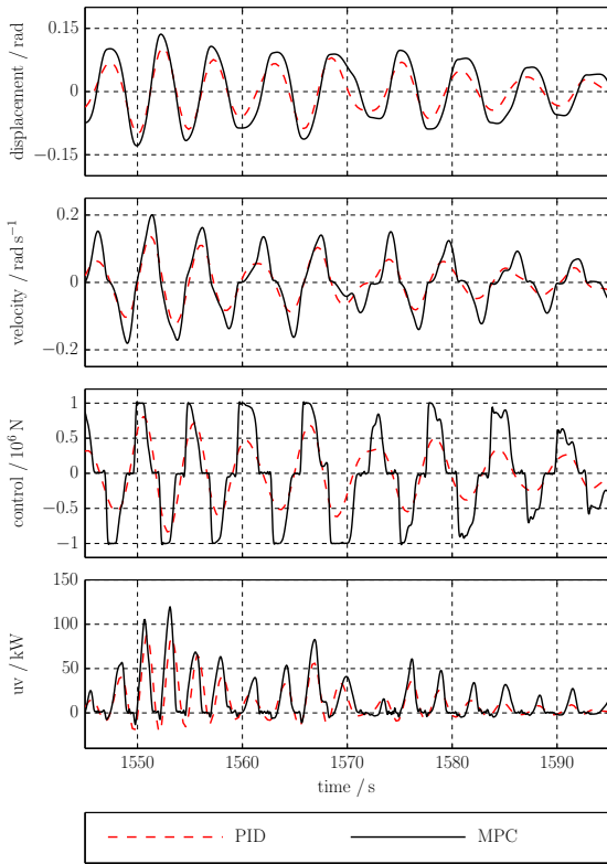
Fig. 13. Comparison of MPC and PI control for the wave 1.
