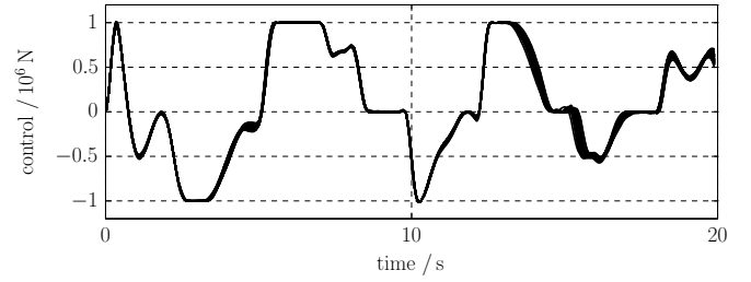
Fig. 5. Optimal control trajectories calculated using random initial values.
