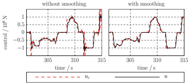
Fig. 4. Impact of the smoothing on the control.
