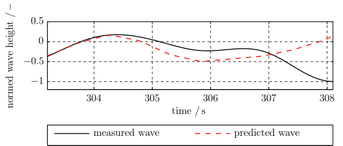
Fig. 12. Wave prediction quality.
