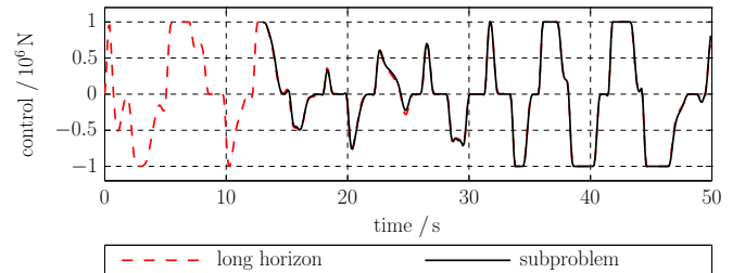
Fig. 7. Verification of the optimum principle: Solution on a sub-interval yields the same trajectory as obtained on the complete interval.
