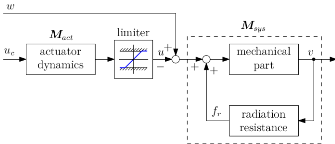
Fig. 2. Structure of the considered mathematical model of the considered machine.
