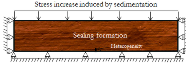
Figure 6. Conceptual model for fracture initiation study and mechanical boundary conditions; the pressure evolution in the reservoir of the basic model is imposed as a boundary condition at the basement of this model
