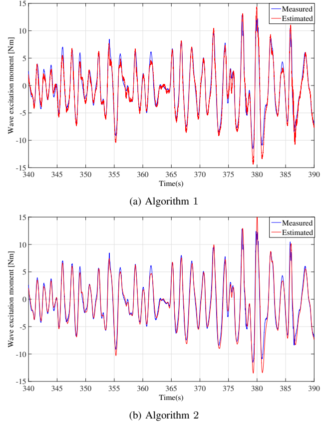
Fig. 8. Measured and estimated wave excitation moments for the transitory period from wave 3 to wave 4.
