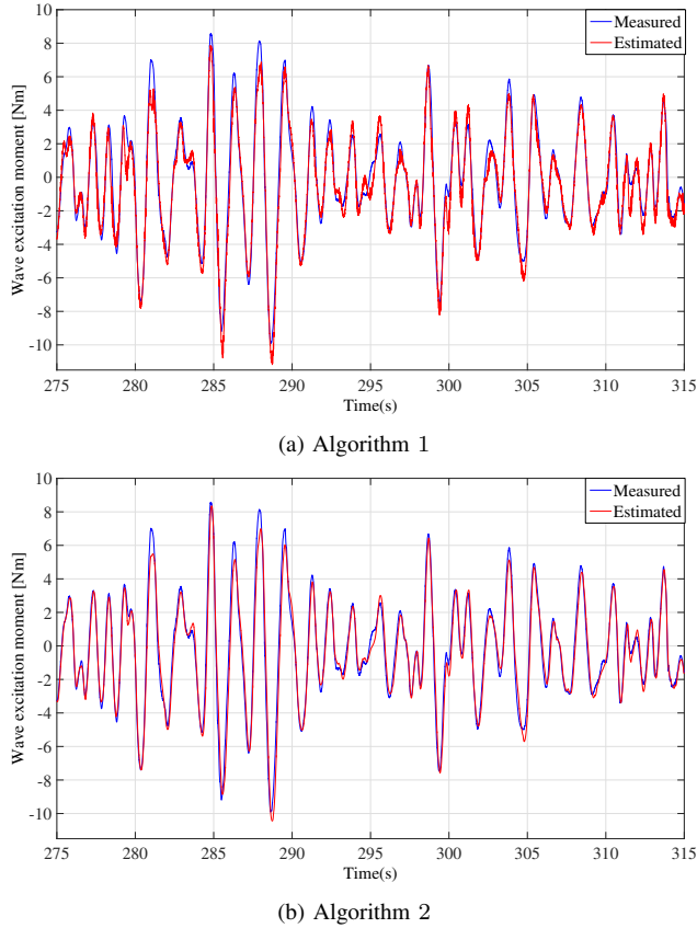
Fig. 7. Measured and estimated wave excitation moments for wave 3.
