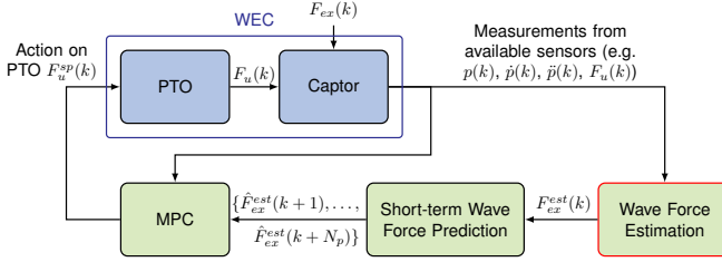
Fig. 2. Wave excitation force estimation in the context of MPC
