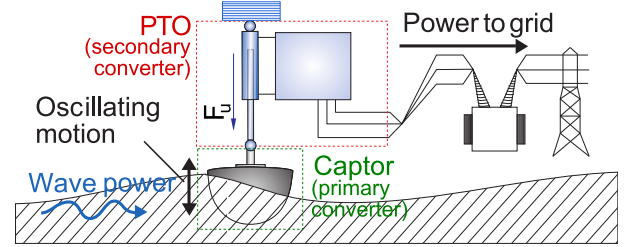
Fig. 1. Schematic diagram of a generic wave energy converter
