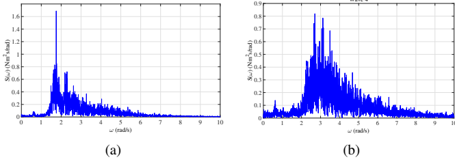
Fig. 6. Spectra of wave 3 and wave 4.
