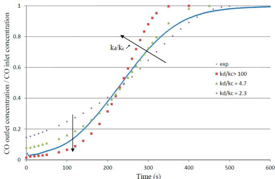
Figure 4. Experimental and simulated (SCM) CO breakthrough curves; k_c = 0.032 \text{ mol}^{-1}\cdot\text{s}^{-1} , test 16.
