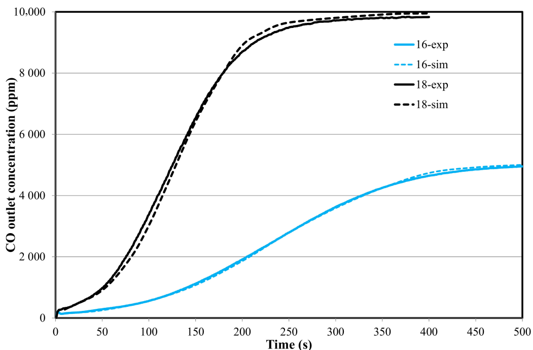
Figure 8. Experimental and simulated breakthrough curves for test 16 (ratio C_0/\text{NiO} = 2.55 ) and for test 18 (ratio C_0/\text{NiO} = 5 ). Operating conditions: T = 800 \text{ }^\circ\text{C} and Q = 40 \text{ NL/h} .
