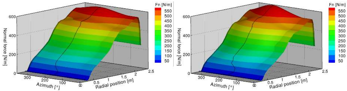
Figure 8: Yawed flow - Surface plot of the normal force against radial position and azimuth, black line indicating the maximum of the normal force at each radial position. U_\infty \approx 18 \text{ m/s} , \Psi \approx 8^\circ (left), U_\infty \approx 15 \text{ m/s} , \Psi \approx 15^\circ (right).
