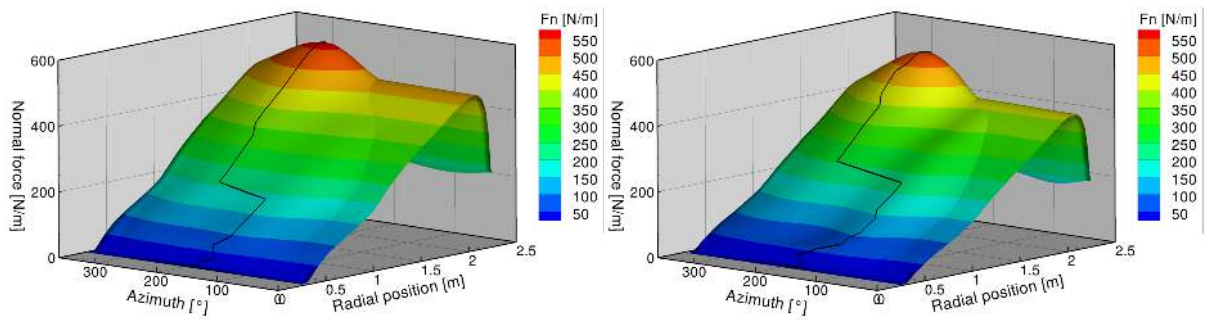
Figure 9: Yawed flow - Surface plot of the normal force against radial position and azimuth, black line indicating the maximum of the normal force at each radial position, U_\infty \approx 15 \text{ m/s} , \Psi \approx 30^\circ (left), U_\infty \approx 15 \text{ m/s} , \Psi \approx 45^\circ (right).
