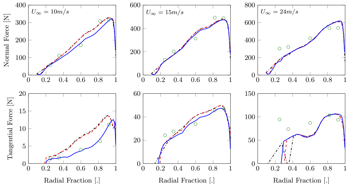
Figure 2. New MEXICO: Normal (top) and tangential (bottom) forces along the blade, wind velocity 10m/s (left), 15m/s (middle) and 24m/s (right). \circ : UAE experiments / —: BEM / - - - : Lifting-Line (Prandtl) / - · - · : Lifting-Line (Mudry)
