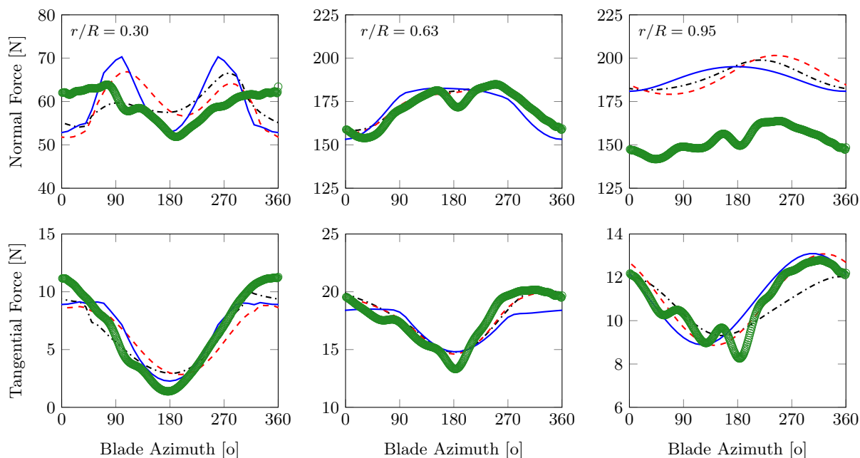
Figure 3. UAE Sequence H: Normal (top) and tangential (bottom) blade loads evolution with azimuth at radial fraction 0.30, 0.63, 0.95, wind velocity 7m/s , yaw angle 20^\circ . \circ : UAE experiments / —: BEM / - - - : Lifting-Line (Prandtl) / . . . : Lifting-Line (Mudry)
