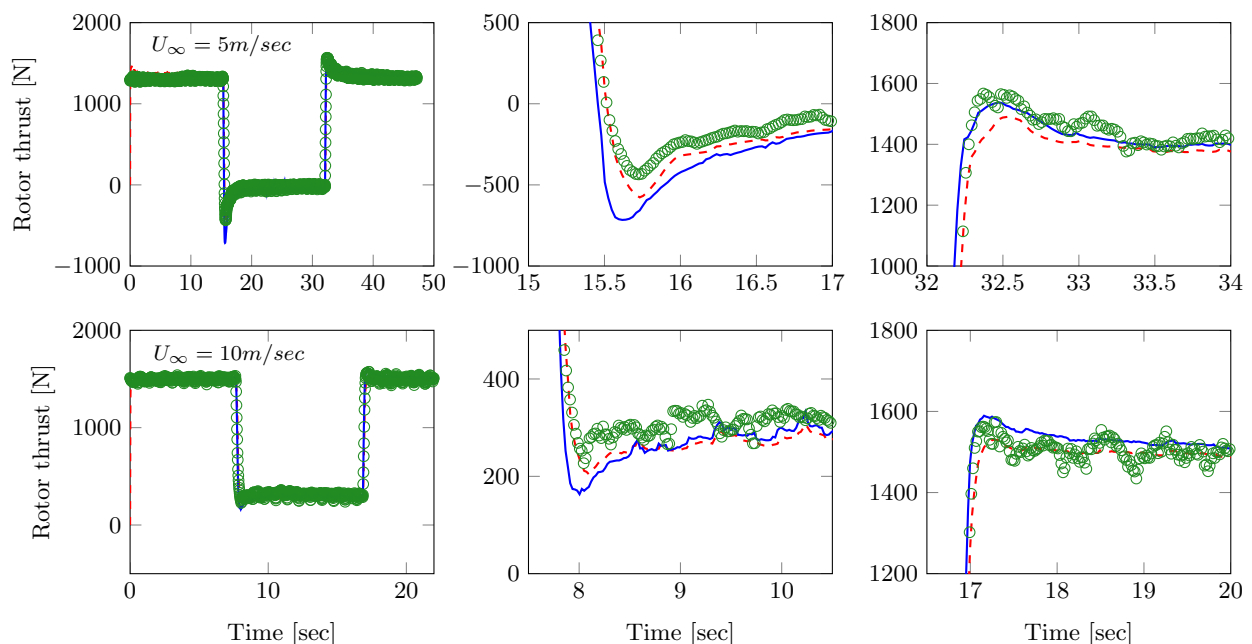
Figure 6. UAE Phase VI: Rotor thrust evolution during pitch steps (left) and close-ups (center and right), wind velocity = 5 m/s (top) and = 10 m/s (bottom). \circ : UAE experiments / — : BEM / - - - : Lifting-Line (Prandtl)
