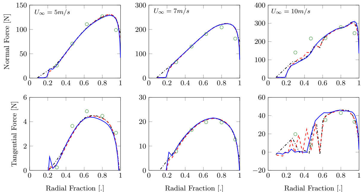
Figure 1. UAE Phase VI, Sequence H: wind velocity 5\text{ m/s} (left), 7\text{ m/s} (middle) and 10\text{ m/s} (right). The green circle \circ represent the UAE experiments, the blue line \text{—} the BEM simulations, the red dashed line \text{---} the Lifting-Line (Prandtl) simulations/ and the black dashed line \text{- - -} the Lifting-Line (Mudry) simulations.
