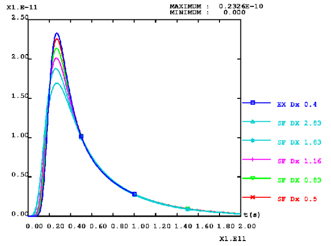
Figure 6. Output mass flux for D_m = 10^{-10} m^2.s^{-1} : influence of \Delta_x .
