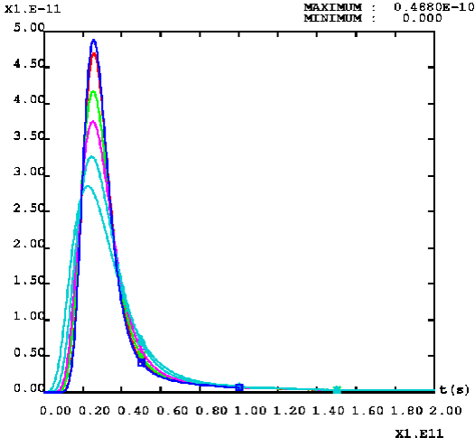
Figure 5. Output mass flux for D_m = 10^{-11} m^2.s^{-1} : influence of \Delta_x .
