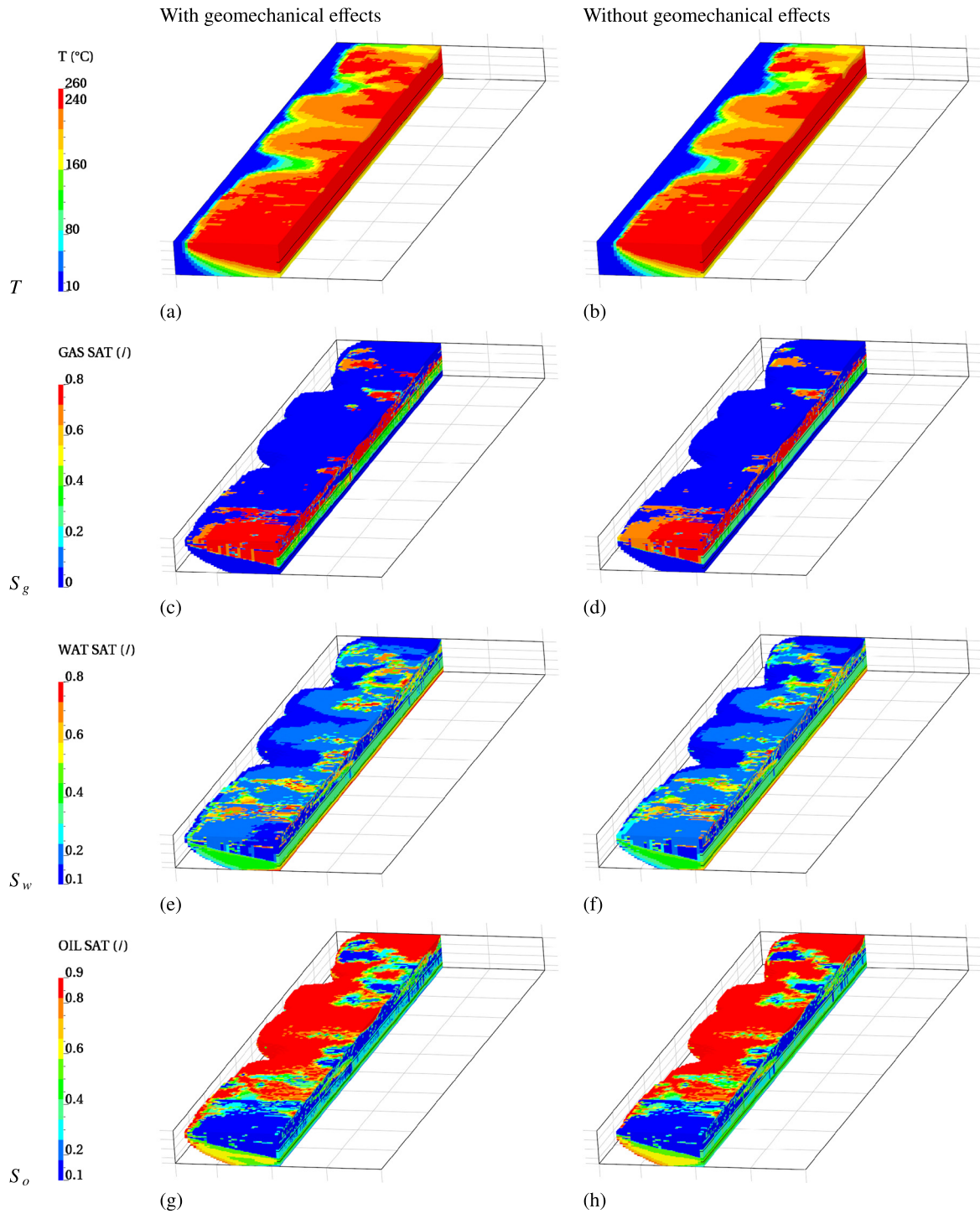
Fig. 3. Field properties in a cut at Y=75 m: T is a temperature, S_g is a gas saturation, S_w is a water saturation and S_o is an oil saturation; upper black line corresponds to the injector well and bottom one to the producer well. Data corresponds to a steam chamber with minimal temperature of 100^{\circ}\text{C} .
