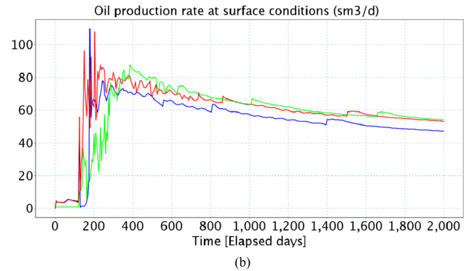
Fig. 5. Cumulative oil production (a) and oil flow rate (b): (red) – with geomechanical effects, (blue) – without geomechanical effects, (green) – without geomechanical effects for the PI calculations only.
