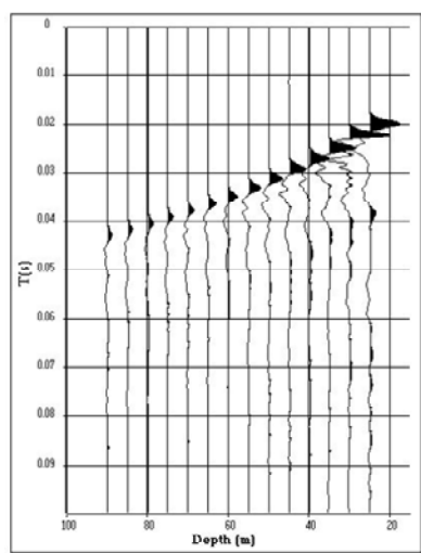
VSP : Raw data (vertical component)
