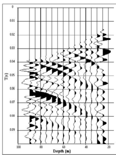
VSP : Up going waves after amplitude recovery
