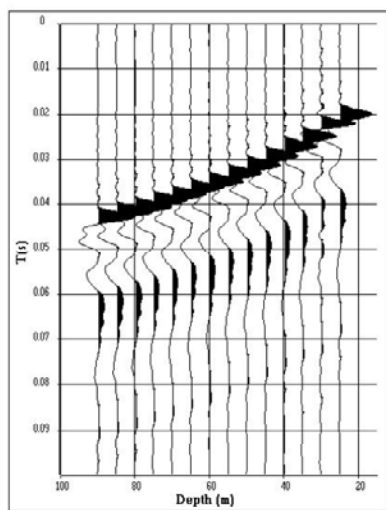
VSP : Down going waves after amplitude recovery
