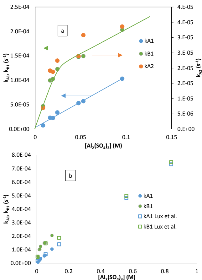
Figure 3: Evolution of the kinetic parameters with Al_2(SO_4)_3 concentration (a: this work at 90°C, lines are guide for the eyes; b: comparison with Lux et al. (T=99°C))
