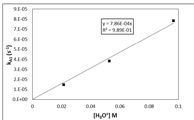
Figure 2: Evolution of k_{A1} kinetic parameter as a function of proton concentration (90°C, addition of H_2SO_4 ).
