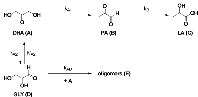
Scheme 1: Proposed reaction mechanism for the conversion of DHA into LA via PA
