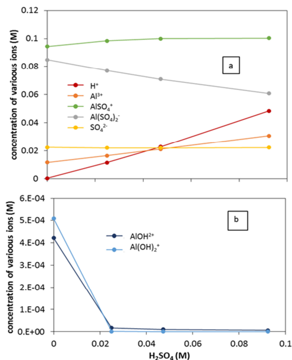
Figure 6: Evolution of the concentration of the different Al cations as a function of H 2 SO 4 concentration calculated using the OLI software (T=90°C, Al 2 (SO 4 ) 3 =0.09 M) (a: H + , Al 3+ and AlSO 4 + ; b: Al(OH) 2+ and Al(OH) 2 + )
