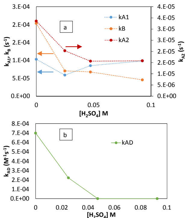
Figure 4: Influence of pH on the kinetic parameters for Al_2(SO_4)_3 aqueous solutions of 0.09 +/- 0.005 M
