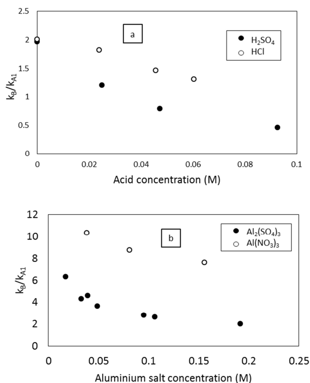
Figure 7: Rate limiting step for the conversion of DHA to LA at T=90°C (a: effect of the addition of acids at Al 2 (SO 4 ) 3 =0.09 M ; b: effect of the concentration of different aluminium salts)
