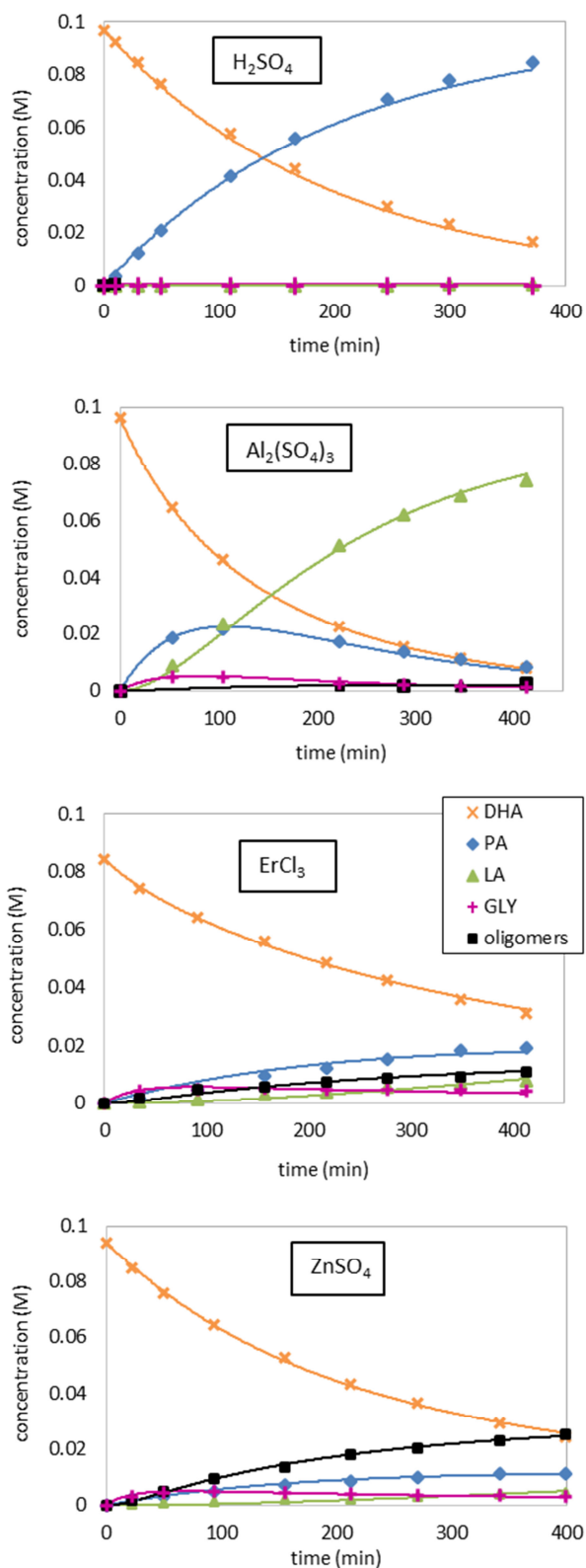
Figure 1: Concentrations profiles as a function of time in the presence of H 2 SO 4 and the different metal salts for the experimental conditions and kinetic parameters specified in Table 1 (points correspond to experiments; lines represent model predictions)
