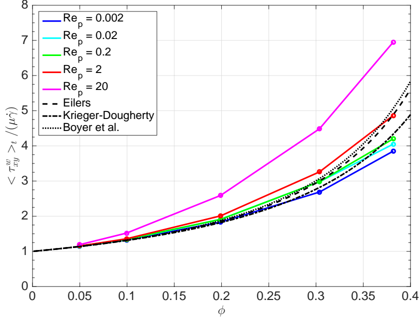
FIG. 5. Variation of the effective viscosity of the suspension, time average of the mean shear stress on walls, \langle \tau_{xy}^w \rangle_t , divided by \mu\dot{\gamma} , with the volume fraction for different particle Reynolds numbers. The dashed line delineates the empirical correlation of Eilers 55 , the dashed-dotted line the correlation of Krieger-Dougherty 2 , and the dotted line, the correlation of Boyer et al. 4 .
