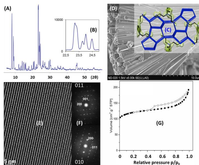
Figure 1. a) XRD pattern of Na-[TPA]-ZSM-5 SAR8 zeolite. The pattern could neither be indexed using the conventional orthorhombic unit cell nor in the monoclinic symmetry; b) Focus on MFI main reflections between 22.5-25°. It is noteworthy that those extra-reflections at smaller 2θ angles can be indexed in the same Pnma space group but with slightly larger unit cell parameters (Table S2); c) Difference electron density map of the two phases showing an electron density cloud that resembled the shape of a TPA + cation located at the intersection of the straight with the sinusoidal 10-ring channels of Na-[TPA]-ZSM-5 SAR8 zeolite. Na + cations were not located in any of the two phases in the refinement, probably because they are disordered. The relative amounts of each phase refined to 71.8 for the main phase (with larger unit cell parameters) and 28.2 for the second phase (with a smaller unit cell). The crystallographic data for this structure are given in Table S2 along with selected interatomic distances and bond angles. The Lorentzian profile fit is shown in Figure S15; d) SEM image of H-ZSM-5 SAR8 zeolite. An assembly into a cauliflower particle having tenths of micrometers in diameter can be observed. It seems that a nodal point served as a starting matter for those elongated needle-like shaped crystals growth; e) HRTEM images of H-ZSM-5 SAR8 sample showing the high regularity of micropore arrays; f) HAADF images confirm the sole formation of the MFI structure; g) Nitrogen adsorption-desorption isotherm for H-ZSM-5 SAR8 zeolite.
