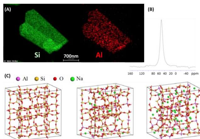
Figure 2. a) TEM EDX mapping of Al, Si elements; b) 27 Al MAS NMR of ZSM-5 SAR8 zeolite; c) Optimized cells calculated by DFT for (a) SAR = ∞, n Al = 0, (b) SAR = 7, n Al = 12, (c) SAR = 2, n Al = 32.
