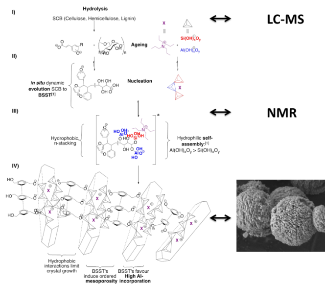
Figure 5. Proposed self-assembly mechanism of aluminate, silicate species and BSST in solution, leading to elongated Al-rich MFI crystals formation.
