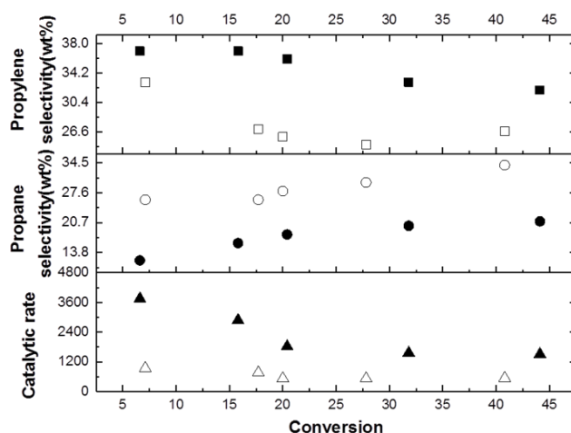
Figure 3. Rate of n-hexane cracking (given in \mu\text{mol}/\text{g}\cdot\text{min}^{-1} ) and selectivities towards propylene and propane (%) as a function of the alkane conversion for ZSM-5 SAR8 and ZSM-5 SAR27. Black and open signs correspond to ZSM-5 SAR8 and SAR27, respectively.
