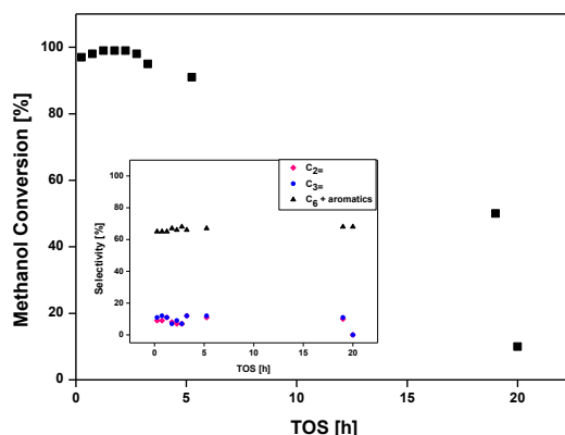
Figure 4. Methanol conversion and selectivity towards hydrocarbons for ZSM-5 SAR8. Conditions: temperature 400°C; WHSV = 1.1 \text{h}^{-1} (Experimental details are given in SI).
