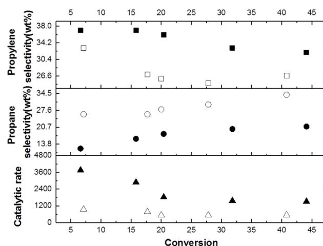
Figure 3. Rate of n-hexane cracking (given in \mu\text{mol/g min}^{-1} ) and selectivities towards propylene and propane (%) as a function of the alkane conversion for ZSM-5 SAR8 and ZSM-5 SAR27. Black and open signs correspond to ZSM-5 SAR8 and SAR27, respectively.
