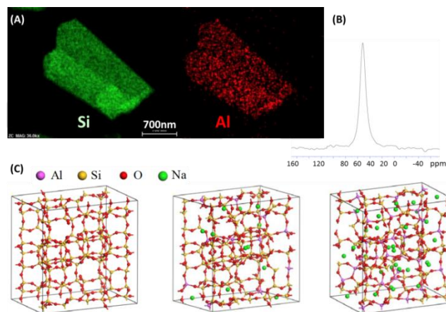
Figure 2. a) TEM EDX mapping of Al, Si elements; b) ^{27}\text{Al} MAS NMR of ZSM-5 SAR8 zeolite; c) Optimized cells calculated by DFT for (a) SAR = \infty , n_{\text{Al}} = 0 , (b) SAR = 7, n_{\text{Al}} = 12 , (c) SAR = 2, n_{\text{Al}} = 32 .
