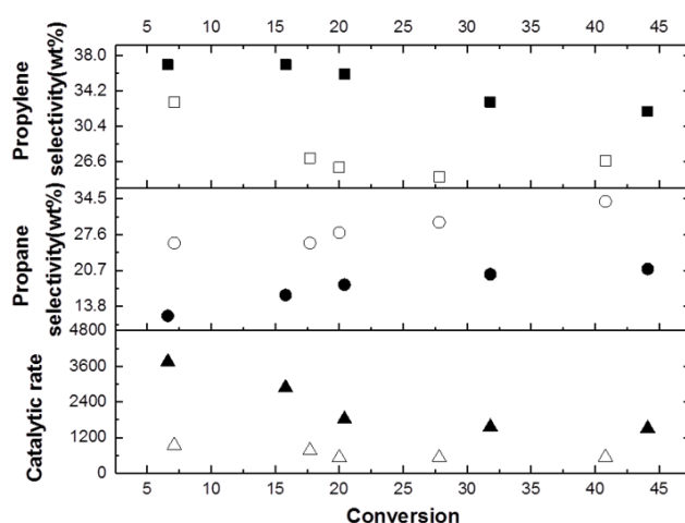
Figure 3. Rate of n-hexane cracking (given in \mu\text{mol}/\text{g} \text{min}^{-1} ) and selectivities towards propylene and propane (%) as a function of the alkane conversion for ZSM-5 SAR8 and ZSM-5 SAR27. Black and open signs correspond to ZSM-5 SAR8 and SAR27, respectively.
