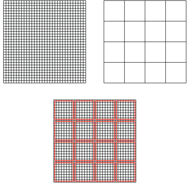
Fig. 1. Construction of the coarse cartesian grid on the right from the fine cartesian grid on the left. In the bottom, the agglomeration is shown.
