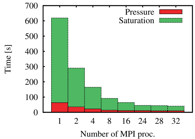
Fig. 10. CPU time used for the resolution of the pressure and saturation equations of the TPFA method on the top and the MMsFE with multiscale global basis functions on the bottom.
