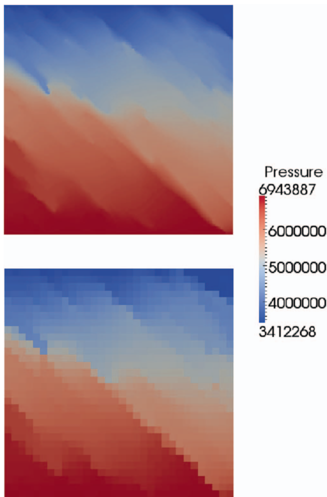
Fig. 15. On the plane z = z_{\max} , pressure solutions (in Pa) of the TPF method on the top and the MMsFE method on the bottom.
