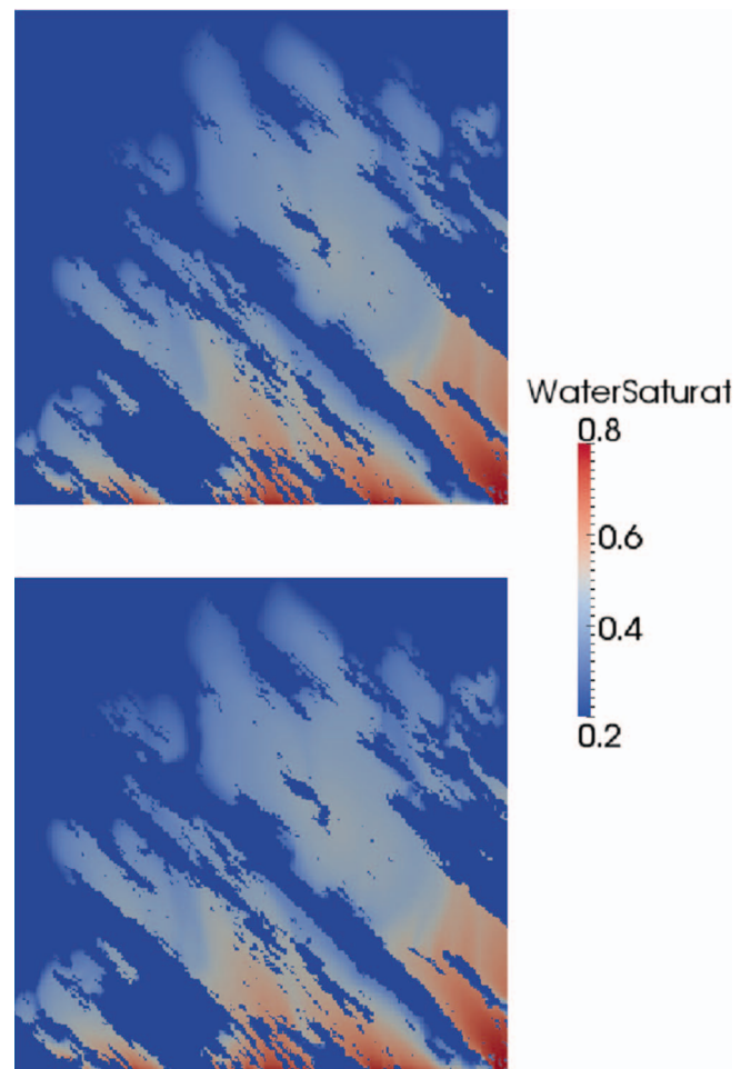
Fig. 16. On the plane z = z_{\max} , water saturation solutions of the TPF method on the top and the MMsFE method on the bottom.
