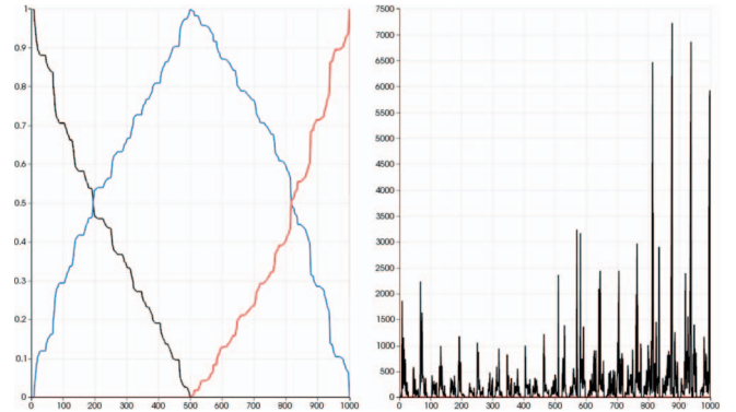
Fig. 3. On the left, 1-d basis functions computed with \mathbf{K} = \mathbf{KId} , \mathbf{K} being represented on the right (in mD).
