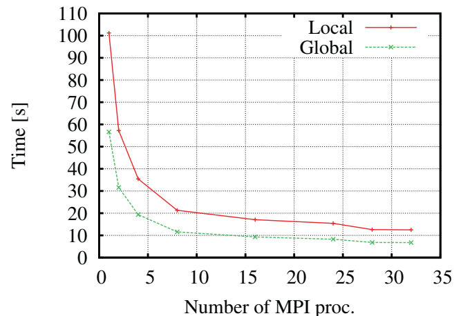
Fig. 8. CPU time used for the calculation of the basis functions.
