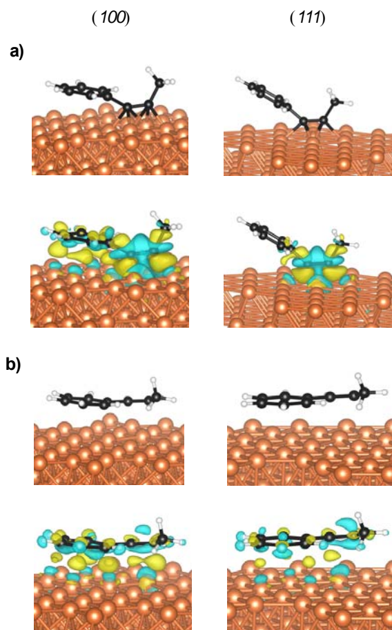
Figure 2. Molecular models for a) S and b) (Z)-S 2 H adsorbed on the (100) and (111) terminations of fcc copper. The bottom pictures show the charge density differences (see method section). Yellow and blue colors represent accumulation or depletion of charge density, respectively. The values for isosurfaces are \pm 2.5 \cdot 10^{-3} \text{ e} \cdot \text{\AA}^{-3} for all models.
