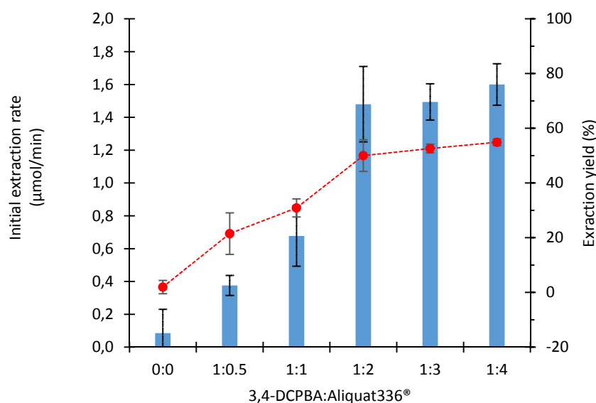
Figure 9. Initial extraction rate in aqueous phase (blue rods) and extraction yield (red dots) in function of 3,4-DCPBA:Aliquat336® molar ratio. [D-Fructose] i = 100 mM, [3,4-DCPBA] = 100 mM, [Aliquat336®] = X mM (X varies from 0 to 400 mM), Tris-HCl
