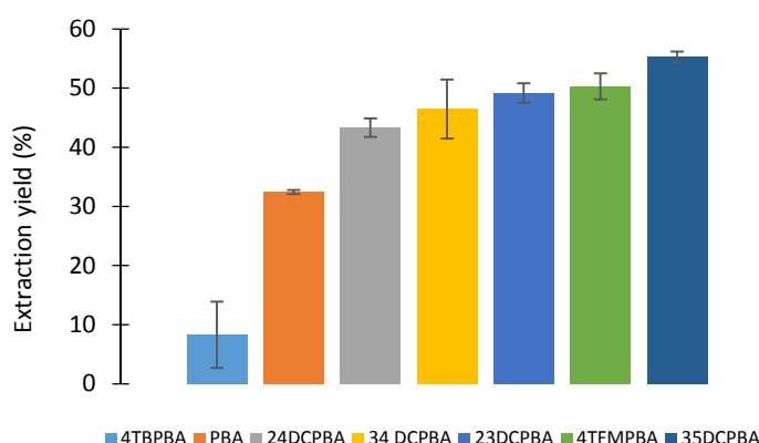
Figure 7. Influence of the arylboronic acid structure on the complexation/transportation process after 45 min. [D-Fructose] I = 100 mM, [Boronic acid] = 100 mM, [Aliquat336®] = 200 mM, Tris HCl 100 mM pH 8.5, MIBK, 343 K, 750 rpm.
