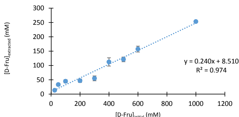
Figure 12. Influence of the initial D-Fructose concentration on the amount of D-fructose extracted. [D-Fructose] I = X mM (X varies from 25 to 1000), [3,4-DCPBA] = 100 mM, [Aliquat336®] = 200 mM, Tris-HCl 100 mM, pH 8.5, MIBK, 343 K, 750 rpm.
