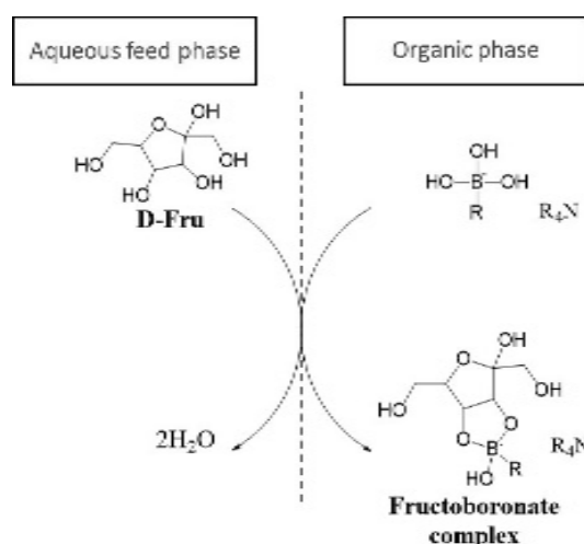
158 Figure 6. Fructoboronate complex formation at the interphase between the first aqueous phase and 159 the organic liquid membrane.
