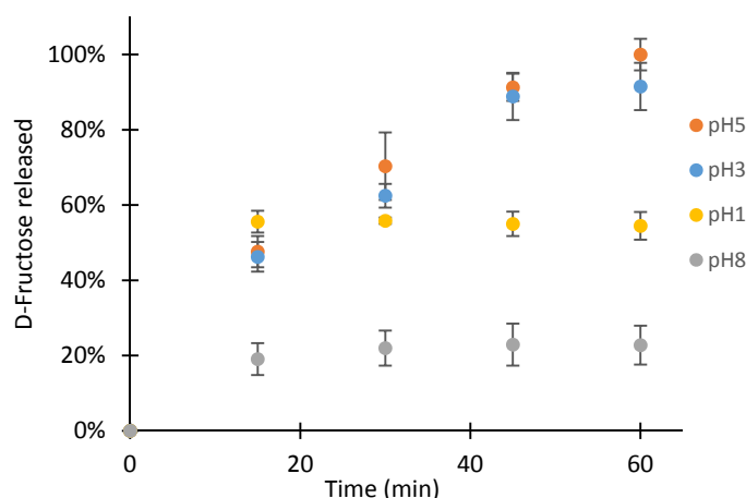
Figure 13. Influence of the pH of the aqueous receiving phase on the D-fructose complex transportation. Extraction process: Tris-HCl 100 mM pH 8.5, [D-Fru]I = 100 mM, [3,4-DCPBA] = 100 mM, [Aliquat336®] = 200 mM, MIBK, 343 K. Receiving phase: Citrate buffer
