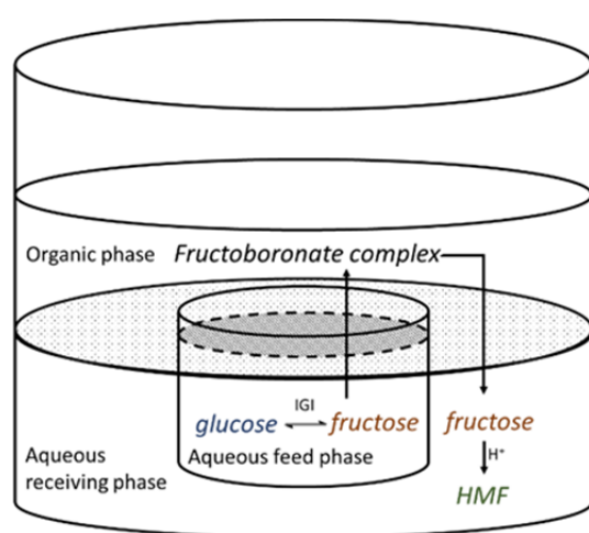
Figure 15. Illustration of the continuous process.
