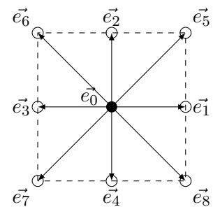
Figure 1. Geometry of the D2Q9 model
