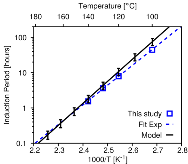
Figure 6: 2-Methylheptane model prediction on IP against present study (blue symbols) and literature data (black symbols). For clarity sake, a regression on present study data (dashed blue line) is performed to assess models (solid black lines) performance. Uncertainty bars represent the IP variation regarding to the oxygen dissolved into liquid. The minimum and maximum respectively corresponds to 50ppm and 2% of initial Oxygen.
