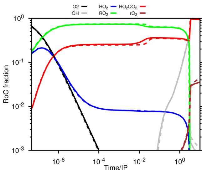
Figure 13: Effect of oxygen concentration on fuel RoC distribution for C8 model. This analysis is conducted at 423 K with 2% and 1000 ppm of oxygen respectively in solid and dashed lines.
