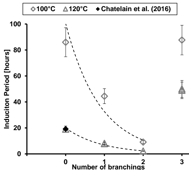
Figure 3: IP variation of several C 8 alkanes as function of temperature and branching level obtained at 373-393 K and 700 kPa of initial oxygen. Uncertainties are calculated including PetroOxy repeatability and compound purity. Exponential regression is presented in dashed lines.
