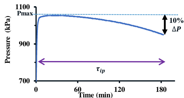
Figure 1: Typical pressure signal obtained during the autoxidation of n-decane e2 at 413 K using a PetroOxy experiment with 700 kPa of initial oxygen.
