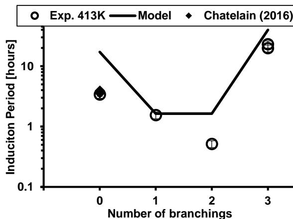
Figure 10: Models prediction of the branching impact on paraffins oxidation kinetics at 413K
