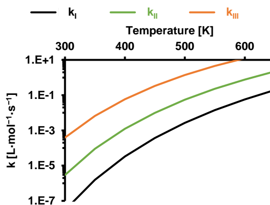
Figure 20: The three different rate constants of the reaction RH + ROO^{\circ} \rightleftharpoons R^{\circ} + ROOH as function of the three different types of hydrogen atoms.
