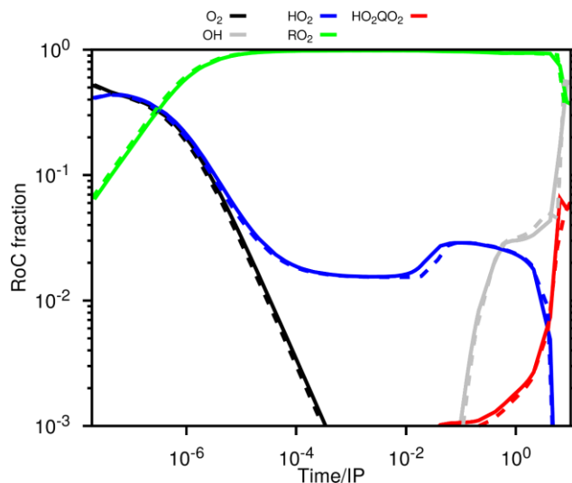
Figure 15: Effect of oxygen concentration on fuel RoC distribution for TMP model. This analysis is conducted at 423 K with 2% and 1000 ppm of oxygen respectively in solid and dashed lines.
