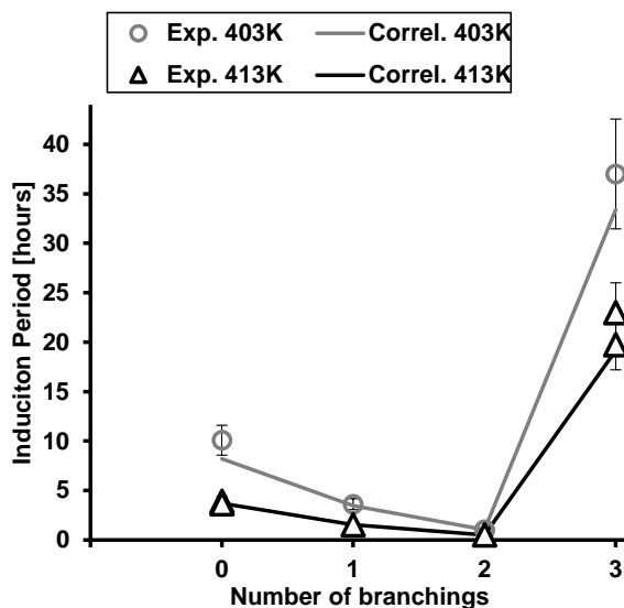
Figure 17: Agreement of correlation prediction with experimental results for both normal and iso-paraffins at two different temperatures. Complementary cases are provided in the supporting material.
