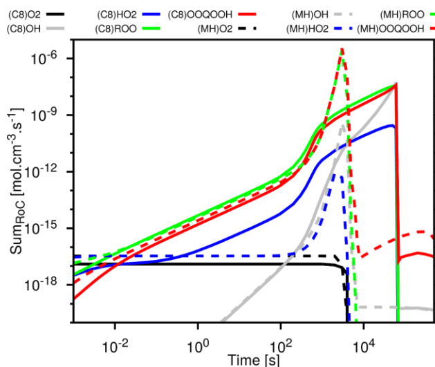
Figure 18: Temporal evolution of the sum of RoC per chemical families at 423K between C8 and MH respectively in solid and dashed lines.
