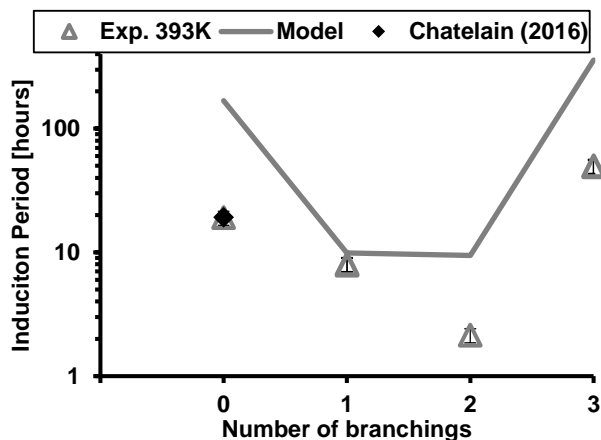
Figure 9: Models prediction of the branching impact on paraffins oxidation kinetics at 393K.
