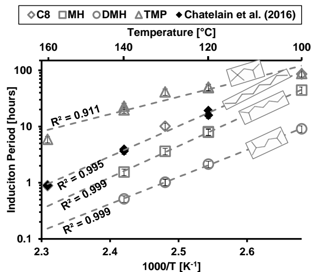
Figure 2: IP measurements obtained with the four molecules obtained at 373-433 K and 700 kPa of initial oxygen. Uncertainties are calculated including PetroOxy repeatability and compound purity. The least-square regression corresponds to the Arrhenius fit IP=A' \times \exp(Ea'/RT) . For which A’ [h] and Ea’/R=Ta’ [K] parameters respectively correspond to: 2.30 \times 10^{-13} and 12.6 for C8, 4.72 \times 10^{-14} and 12.9 for MH, 1.24 \times 10^{-12} and 11.1 for DMH, 6.65 \times 10^{-7} and 7.1 for TMP.
