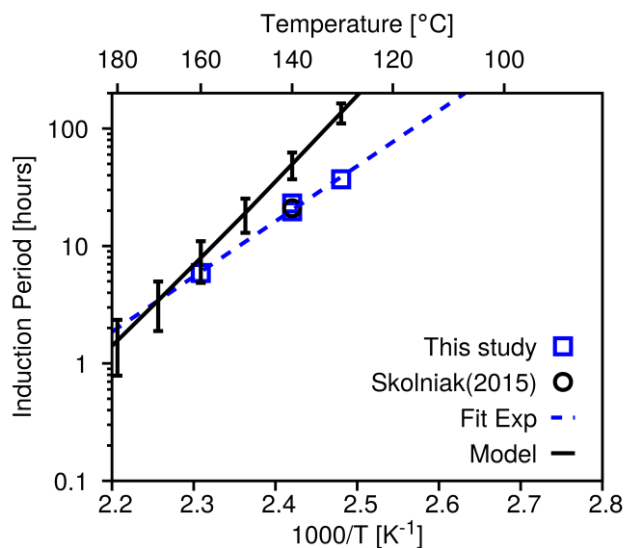
Figure 8: 2,2,4-trimethylpentane model prediction on IP against present study (blue symbols) and literature data (black symbols). For clarity sake, a regression on present study data (dashed blue line) is performed on the high temperature regime only to assess models (solid black lines) performance. Uncertainty bars represent the IP variation regarding to the oxygen dissolved into liquid. The minimum and maximum respectively corresponds to 50ppm and 2% of initial Oxygen.
