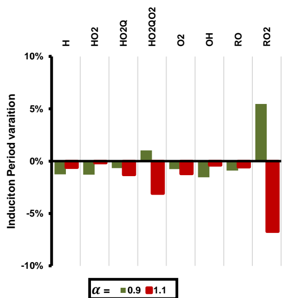
Figure 16 : Relative IP variation according to a specific enhancement factor ( \alpha ) for a given reaction family. A 10% variation of the initial pre-exponential factor was applied on the following eight “fuel+X” reaction families with X = H^\circ, HO_2^\circ, HO_2Q^\circ, HO_2QO_2^\circ, O_2, OH^\circ, RO^\circ, RO_2^\circ .
