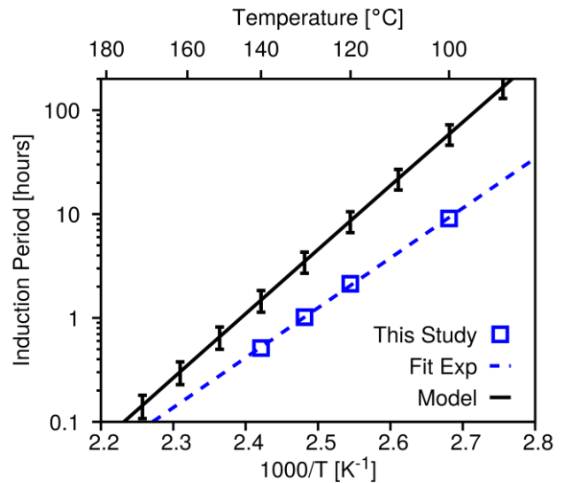
Figure 7: 2,5-dimethylhexane model prediction on IP against present study (blue symbols) and literature data (black symbols). For clarity sake, a regression on present study data (dashed blue line) is performed to assess models (solid black lines) performance. Uncertainty bars represent the IP variation regarding to the oxygen dissolved into liquid. The minimum and maximum respectively corresponds to 50ppm and 2% of initial Oxygen.
