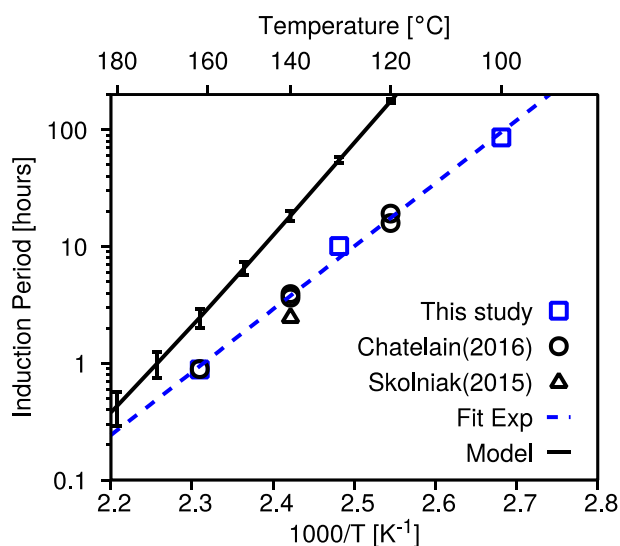
Figure 5: N-octane model prediction on IP against present study (blue symbols) and literature data (black symbols). For clarity sake, a regression on present study data (dashed blue line) is performed to assess models (solid black lines) performance. Uncertainty bars represent the IP variation regarding to the oxygen dissolved into liquid. The minimum and maximum respectively corresponds to 50 ppm and 2 % of initial oxygen.
