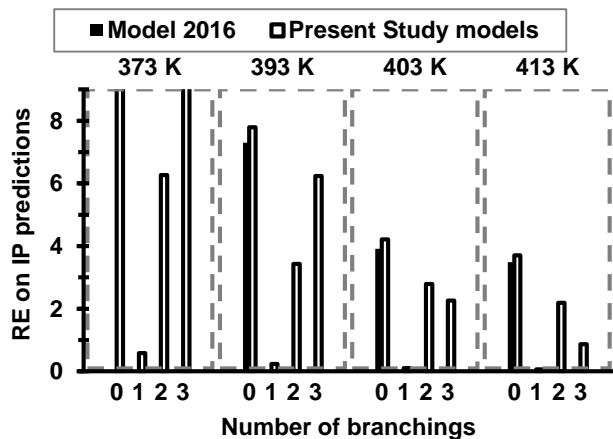
Figure 11: Relative Errors (RE) for both present and literature data models to predict the Induction Periods (IP) at several temperatures. Models with 0 and 3 branchings at 373 K are out of the scale and respectively have a RE of 24 and 47.
