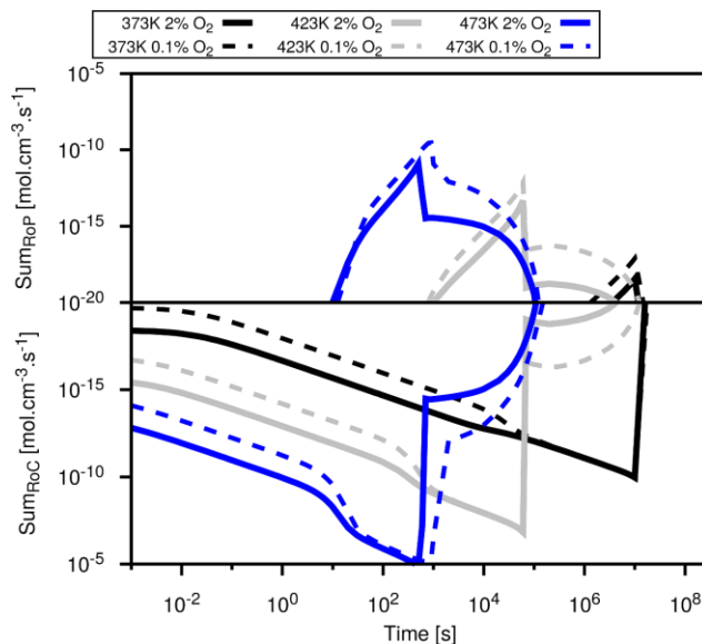
Figure 12: Sum of RoC/RoP on fuel consumption for the C_8 mechanism at 373 K, 423 K and 473 K.
