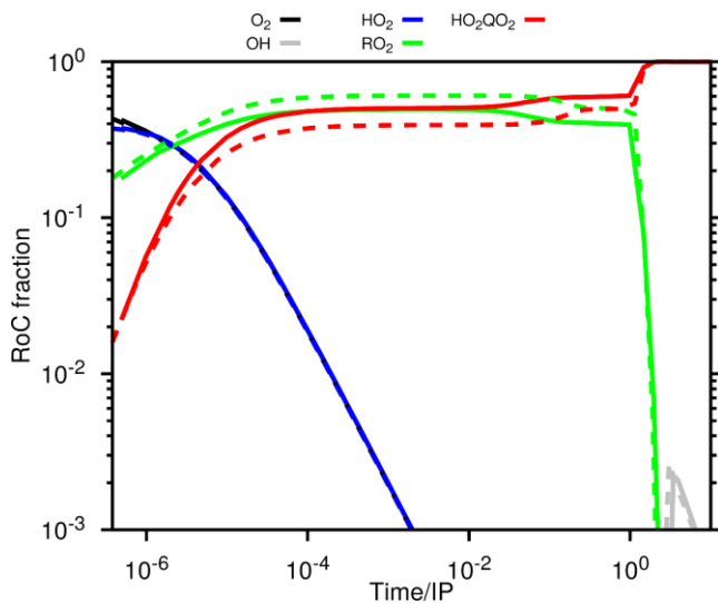
Figure 14: Effect of oxygen concentration on fuel RoC distribution for MH model. This analysis is conducted at 423 K with 2% and 1000 ppm of oxygen respectively in solid and dashed lines. r\text{OO}^\circ stands for the sum of light hydroperoxides from C_1 to C_7
