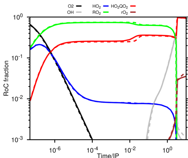
Figure 13: Effect of oxygen concentration on fuel RoC distribution for C8 model. This analysis is conducted at 423 K with 2% and 1000 ppm of oxygen respectively in solid and dashed lines.
