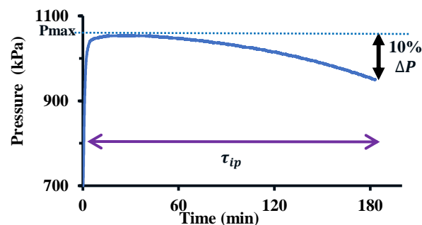
Figure 1: Typical pressure signal obtained during the autoxidation of n-decane 12 at 413 K using a PetroOxy experiment with 700 kPa of initial oxygen.
