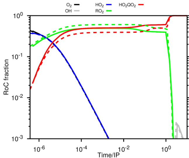
Figure 14: Effect of oxygen concentration on fuel RoC distribution for MH model. This analysis is conducted at 423 K with 2% and 1000 ppm of oxygen respectively in solid and dashed lines. r\text{OO}^\circ stands for the sum of light hydroperoxides from \text{C}_1 to \text{C}_7 .
