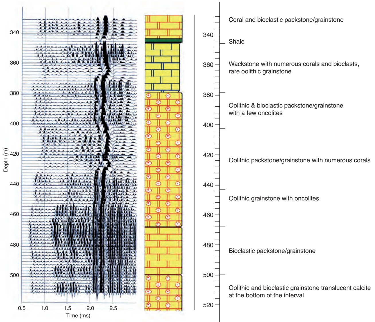
Figure 4 Acoustic logging and lithological description (Courtesy of Andra).
