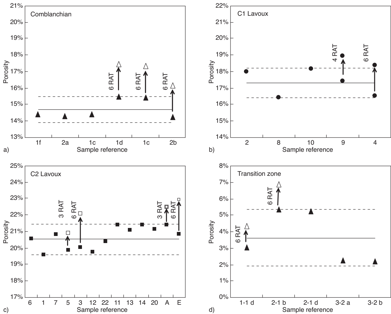
Figure 7 Sample porosity before and after alteration.
