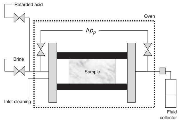
Figure 3 Experimental device for homogeneous alteration of the rock samples.
