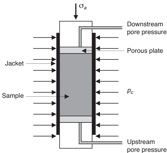
Figure 8 Principle of a triaxial test.
