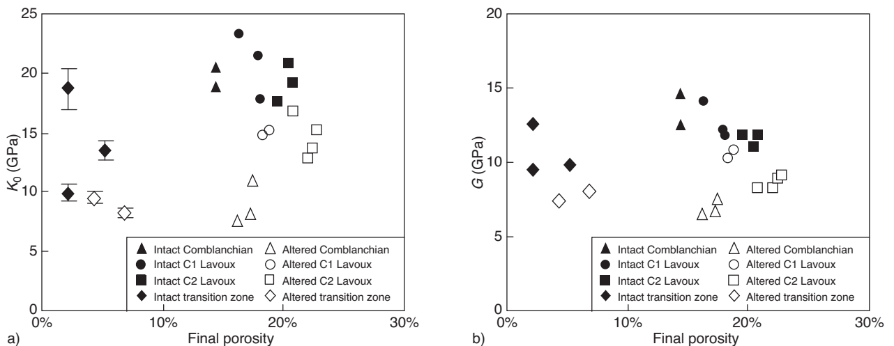
Figure 10 Drained elastic moduli of intact and altered samples.
