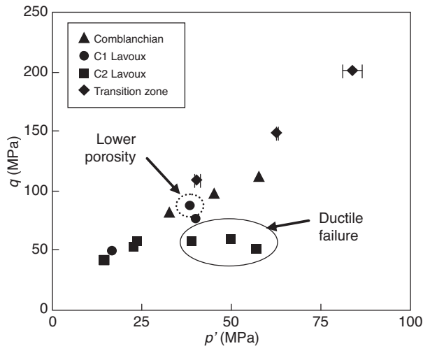
Figure 9 Failure points of intact samples.
