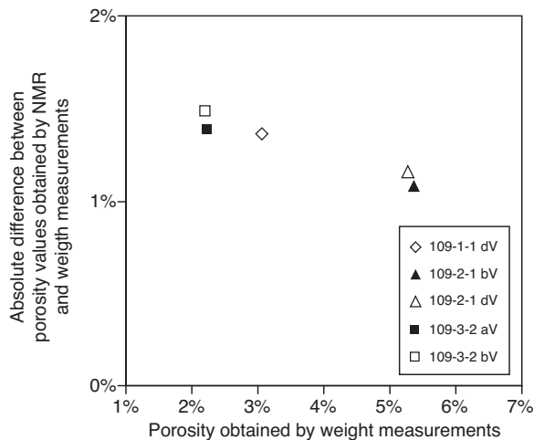
Figure 2 Absolute difference between porosity values obtained through NMR and weight measurements for transition zone samples.
