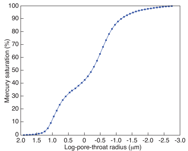
Figure 2 Mercury porosimeter results.
