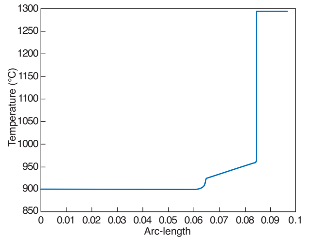
Figure 13 Temperature profile at the bottom of the SMR reactor.
