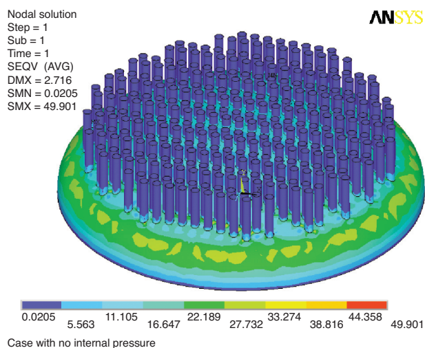
Figure 14 Von Mises stresses (MPa).
