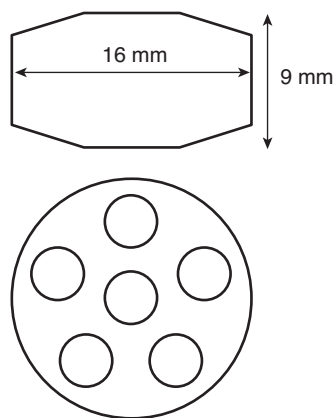
Figure 18 BASF SG-9301 catalyst.
