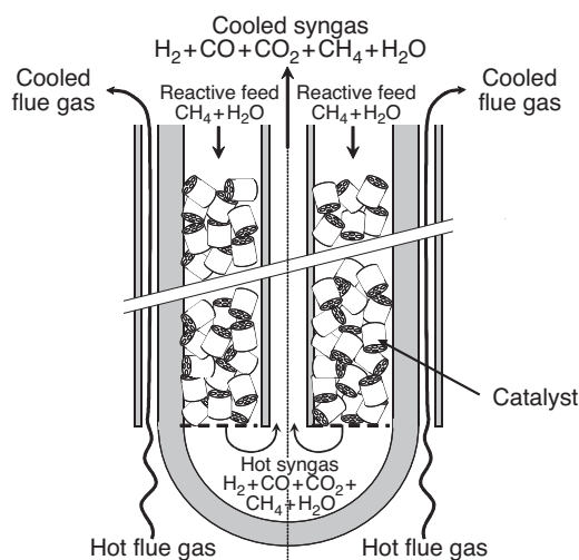
Figure 7 Bayonet tube concept.
