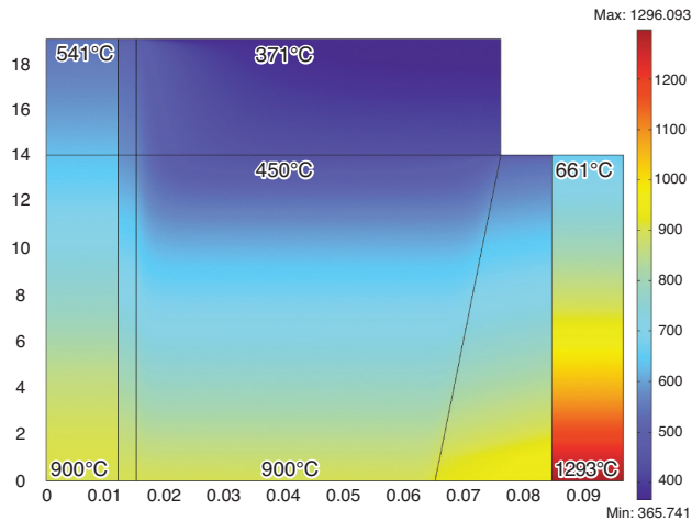
Figure 11 Temperature map in the SMR reactor.
