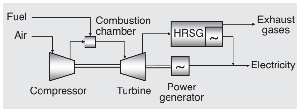
Figure 1 Simplified combined cycle gas turbine scheme.
