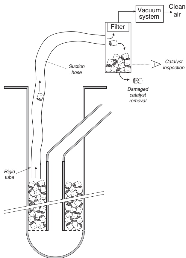
Figure 20 Catalyst unloading.
