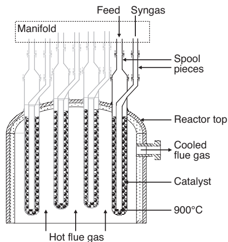
Figure 8 Reactor arrangement concept.
