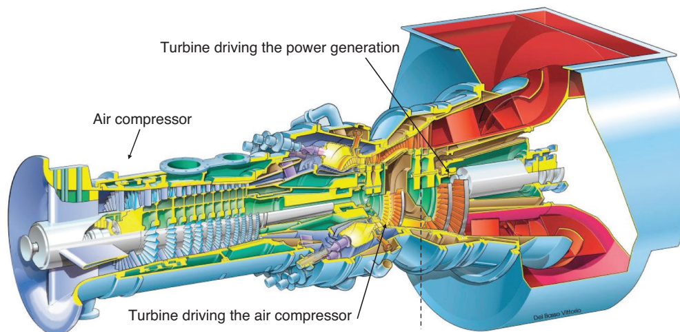
Figure 2 SGT-700 Core Engine (dashed line: transition between the two parts of the turbine).
