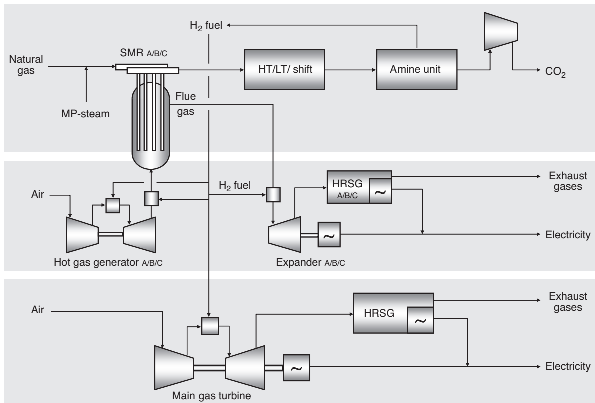
Figure 6 Schematic representation of HyGenSys-1.
