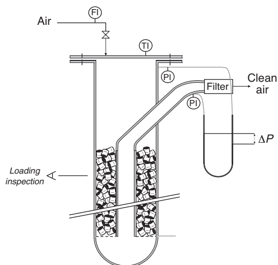
Figure 19 Pressure drop measurement.
