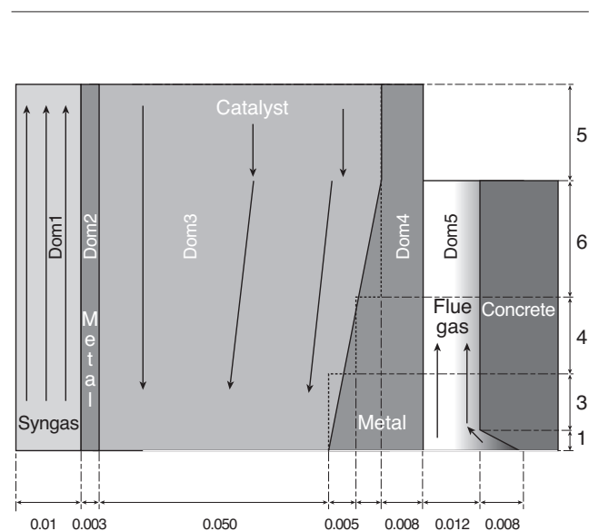
Figure 9 SMR reactor tube geometry.
