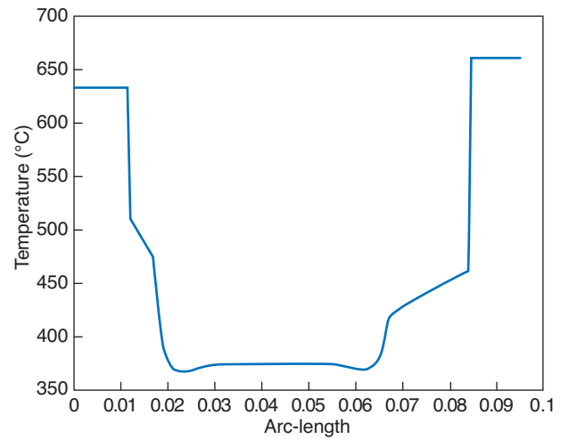
Figure 12 Temperature profile at the top of the SMR reactor.
