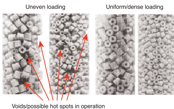
Figure 15 Comparison between uneven loading and uniform loading.
