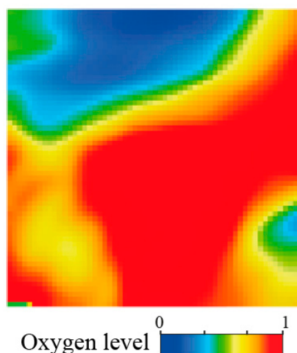
Figure 12. Oxygen level at sea-floor map for a meta-model with a high oxygen mixing rate (0.98) and a fairly high PP0 ( 225 \text{ gC} \cdot \text{m}^{-2} \cdot \text{year}^{-1} ). We can expect anoxic environments in the blue areas that correspond to the deepest parts of the basin. With this setting, the anoxia is only driven by the high amount of primary productivity.
