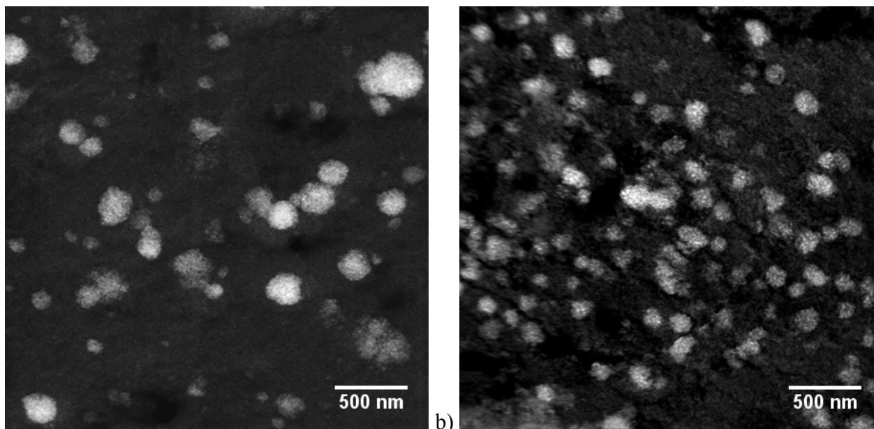
443 a) b) 444 Figure 5 : HAADF-STEM images of a) oxide catalyst ; b) reduced catalyst. 445
