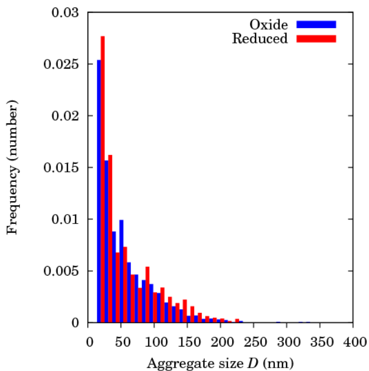
446 447 Figure 6 : Cobalt aggregates size distribution, measured by HAADF-STEM, expressed by number 448 frequency: in oxide catalyst (blue) and reduced catalyst (red) 449
