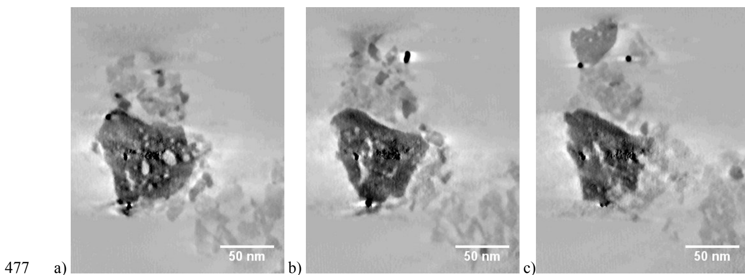
478 Figure 11 : a-c) Slices from electron tomography reconstructions for a cobalt aggregate in the oxide 479 catalyst.
