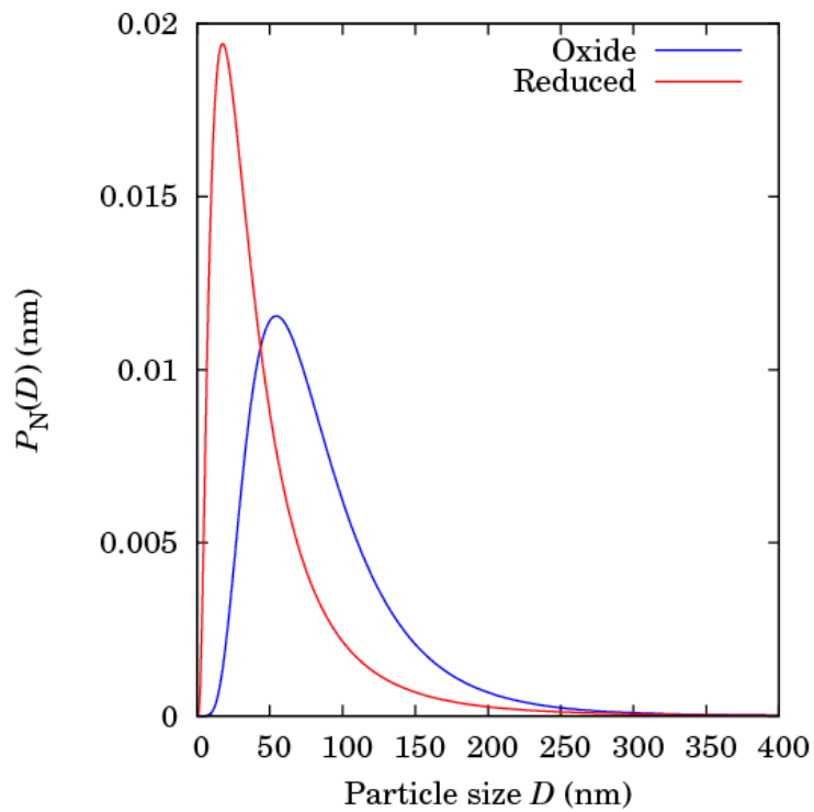
450 451 Figure 7 : Number aggregates size distribution ( P_N ) obtained by ASAXS for the oxide and the 452 reduced catalysts. 453
