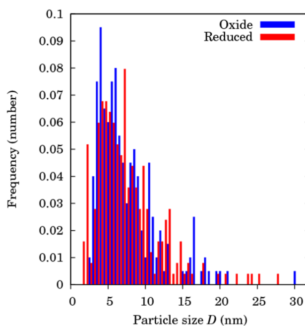
396 a) Dark-field TEM image of oxide Co/silica-alumina. b) Particles size distribution 397 expressed by number frequency: in oxide catalyst (blue) and reduced catalyst (red) 398
