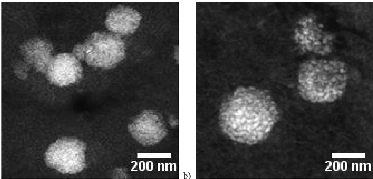
454 a) b) 455 Figure 8 : High magnification HAADF-STEM images of a) oxide catalyst ; b) reduced catalyst. 456
