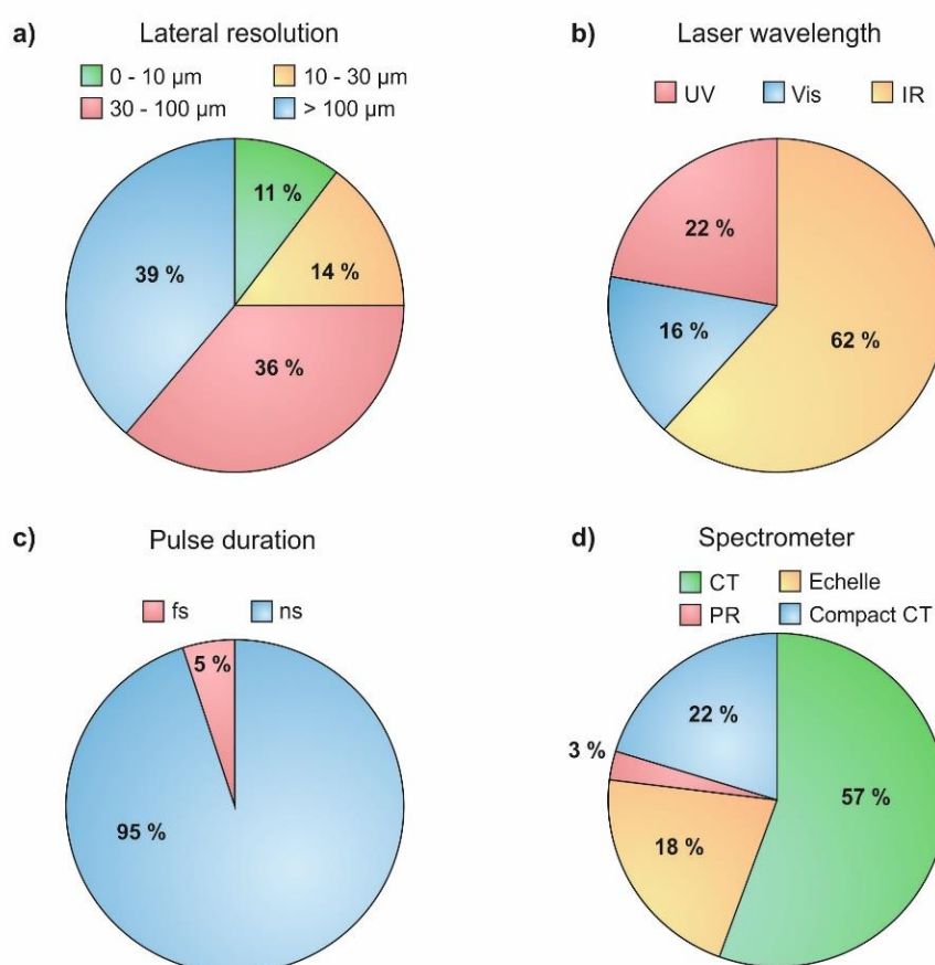
Fig. 2. Configurations used for LIBS-based imaging since 2012. a) Spatial resolution ranges. b) Laser wavelengths and c) pulse durations. d) Types of spectrometers. CT: Czerny Turner spectrometer, PR: Pashen Runge spectrometer.
