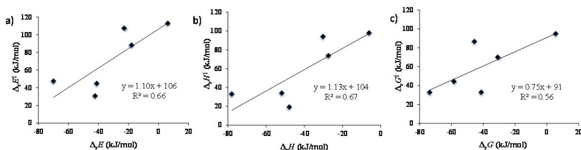
Figure 9. Brønsted–Evans–Polanyi (BEP) linear relationships based on a) electronic energy, b) enthalpy, c) free energy for C-H bond cleavage steps at PBE-dDsC level
