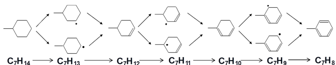
Figure 2. Simplified network for the dehydrogenation of MCH into toluene via 4-methyl-cyclohexene (4-MCHe) and methyl-cyclohexadiene (MCHde) intermediates.
