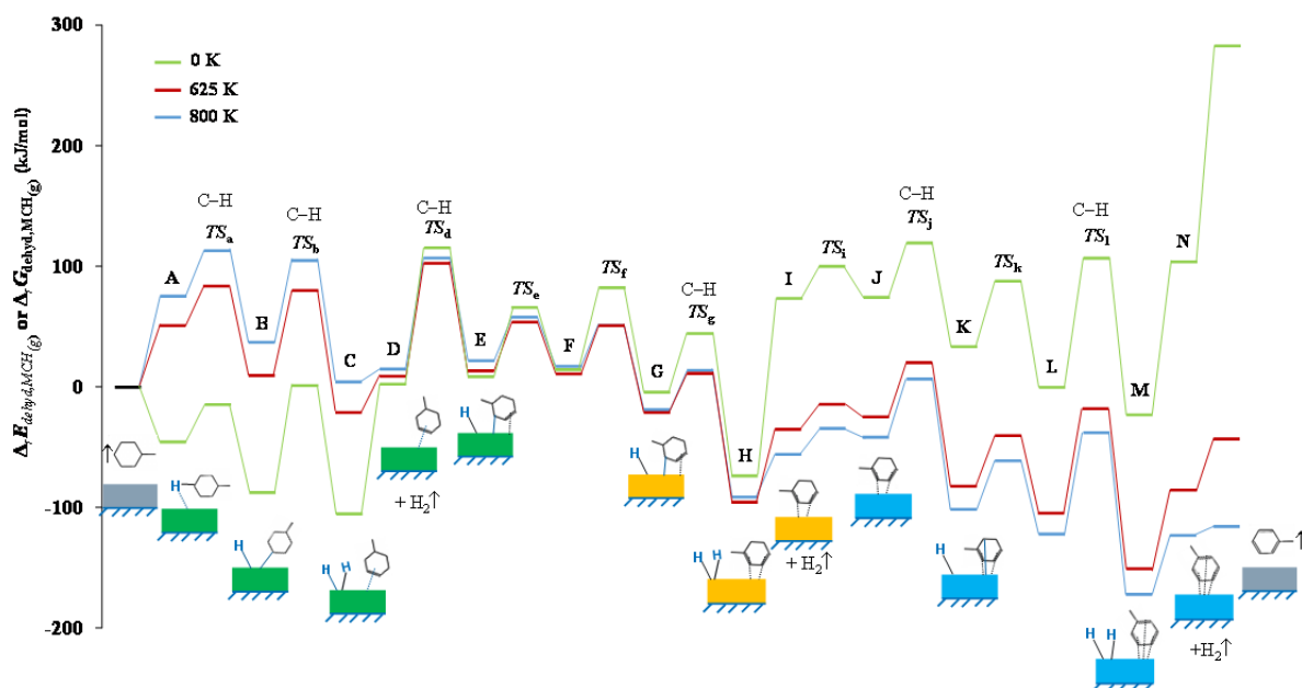
Figure 4. Free energy profile (PBE-dDsC level) for methyl-cyclohexane dehydrogenation over \text{Pt}_{13}\text{H}_6/\gamma\text{-Al}_2\text{O}_3 at 625 K and 800 K along with the corresponding electronic energy profiles at 0 K. Each colored box represents the cluster with 6 H atoms and various colors correspond to different cluster morphologies (highlighted in Figures 5 and 6 with the same color coding).
