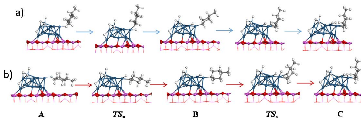
Figure 8. Comparison of the first five intermediates and transition states optimized by using a) PBE and b) PBE-dDsC functionals
