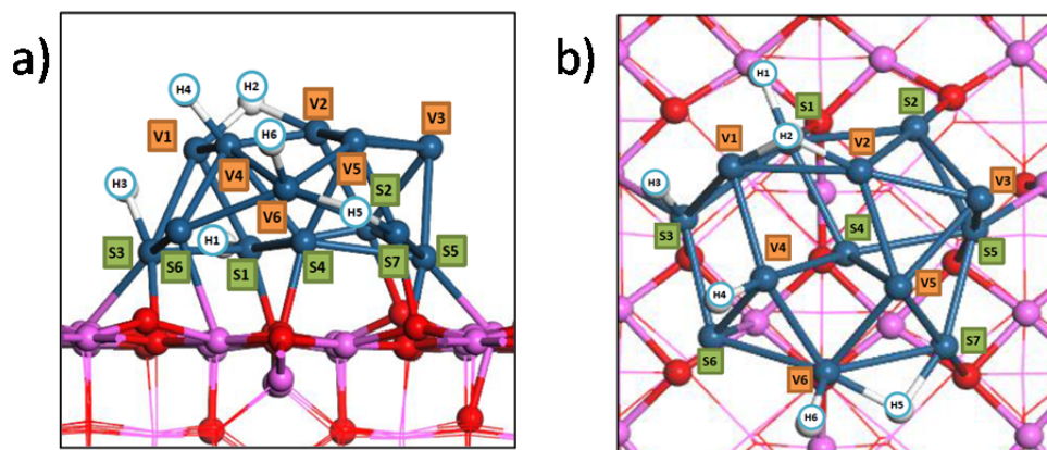
Figure 1. Molecular structure of the starting model of Pt 13 /γ-Al 2 O 3 (100) with 6 adsorbed hydrogen atoms. a) side view, b) top view. Pt atoms labelled with letter “S” are located at the alumina surface, Pt atoms labelled with letter “V” are in contact with vacuum. Color legend: aluminum (pink balls), oxygen (red balls), platinum (dark blue balls), hydrogen (white balls)
