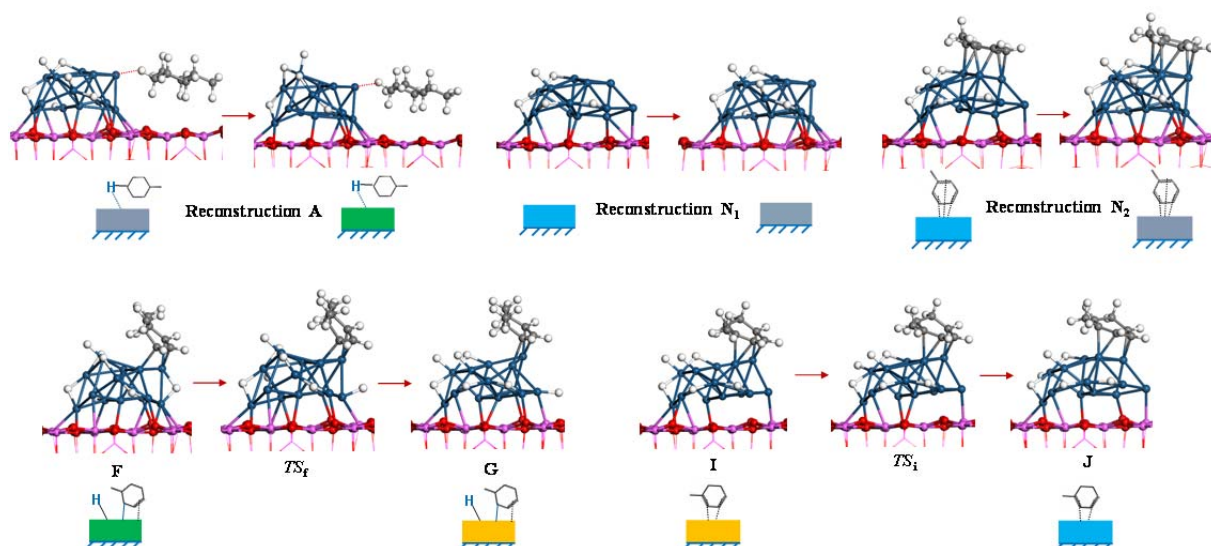
Figure 6. Molecular structures along the cluster reconstruction steps (PBE-dDsC level). Color legend: aluminum (pink balls), oxygen (red balls), platinum (dark blue balls), carbon (dark grey balls), hydrogen (white balls)
