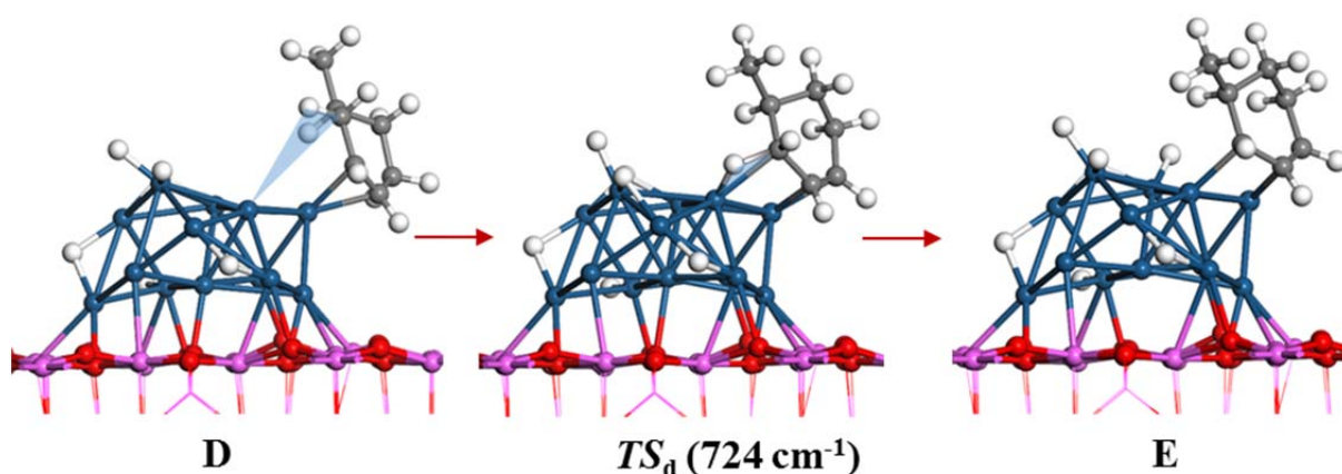
Figure 7. Molecular structure of intermediate methyl-cyclohexene ( D ) leading to intermediate methyl-cyclohexenyl+H ( E ) through the TS_d transition state. The blue triangle represents the 3 centers complex (C-H-Pt) involved during the C-H scission. The unique imaginary frequency at TS_d is given in parenthesis. Color legend: aluminum (pink balls), oxygen (red balls), platinum (dark blue balls), carbon (dark grey balls), hydrogen (white balls)
