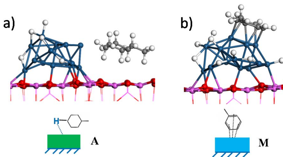
Figure 5. a) Adsorption mode of (A) methyl-cyclohexane and b) of (M) toluene on \text{Pt}_{13}\text{H}_6/\gamma\text{-Al}_2\text{O}_3 . Color legend: aluminum (pink balls), oxygen (red balls), platinum (dark blue balls), carbon (dark grey balls), hydrogen (white balls)
