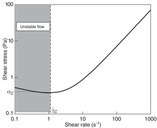
Figure 6 Steady State behavior of a virtual fluid.
