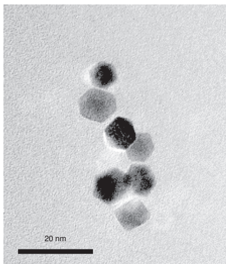
Figure 4 TEM characterization of Pt-polyhedron Sol after 3 hours of ageing.
