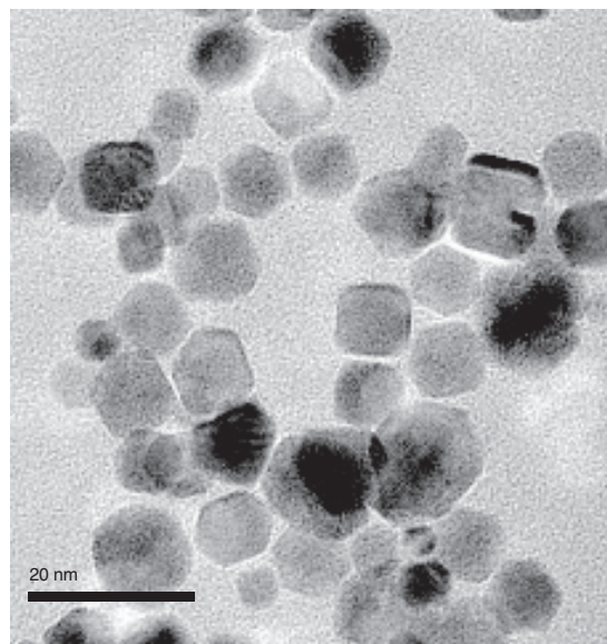
Figure 5 TEM characterization of Pt-Mix Sol after 3 hours of ageing.
