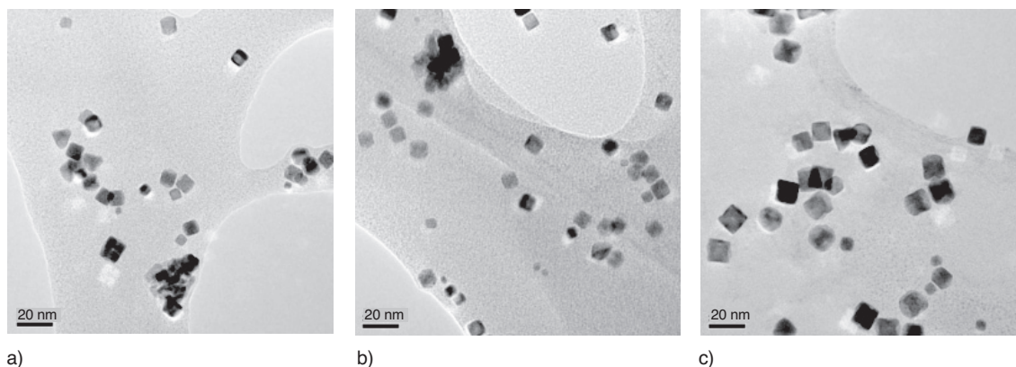
Figure 8 TEM characterization of Pt-Mix sol after 5 a), 10 b) and 16 min c).
