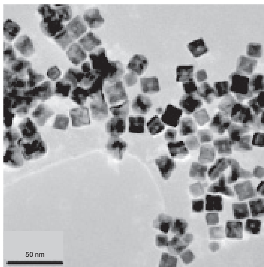
Figure 6 TEM characterization of Pt-cube sol after 3 hours of ageing.
