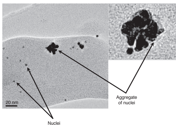
Figure 7 TEM characterization of Pt-Mix sol after 2 min.
