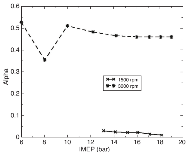
Figure 10 Evolution of the parameter as a function of the expected IMEP (bar).
