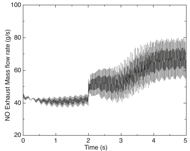
Figure 19 NO exhaust mass flow rate.
