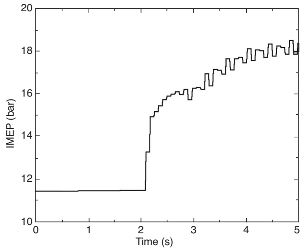
Figure 15 Evolution of the simulated IMEP during the transient engine simulation.
