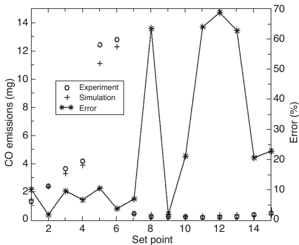
Figure 12 Experimental and simulated CO emissions.
