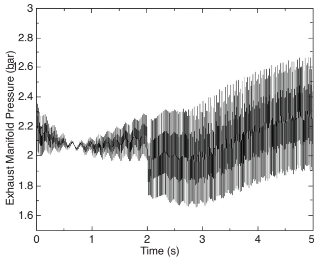
Figure 17 Evolution of the exhaust manifold pressure.
