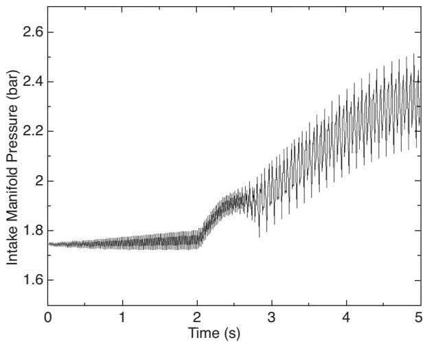
Figure 16 Evolution of the intake manifold pressure.
