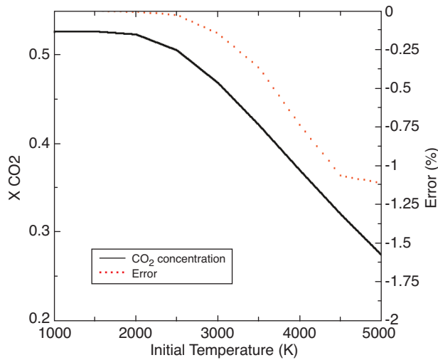
Figure 4 Evolution of CO 2 concentration.
