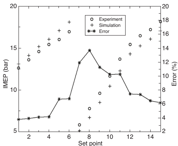
Figure 11 Experimental and simulated IMEP.
