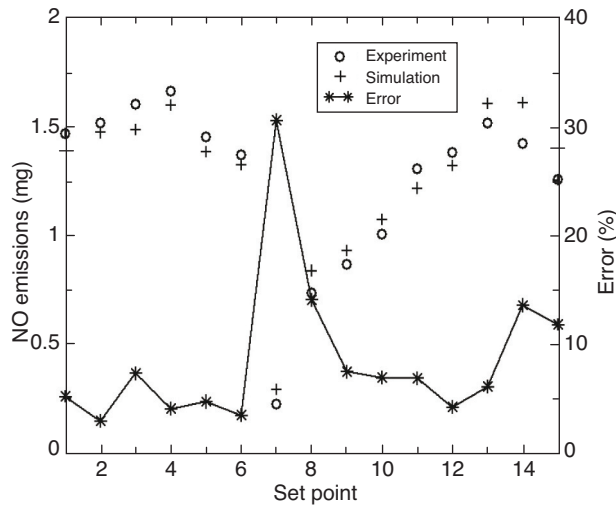
Figure 13 Experimental and simulated NO emissions.
