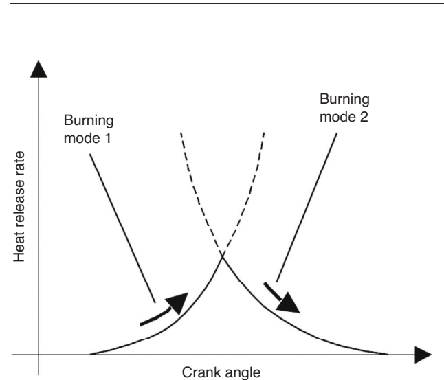
Figure 3 Pre-mixed combustion model (from [1]).
