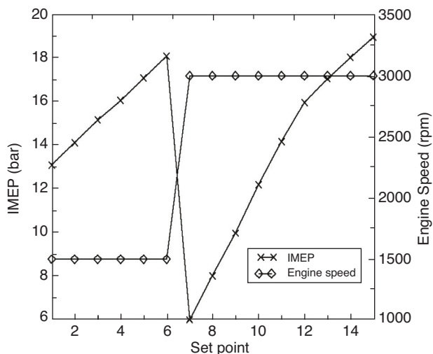
Figure 9 IMEP and engine speed of the 15 set points.
