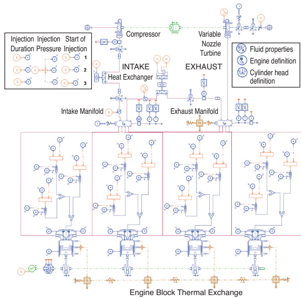
Figure 14 Diesel engine simulator.
