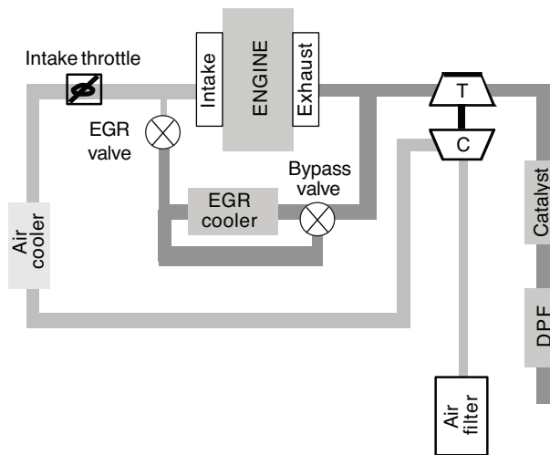
Figure 7 Engine architecture.
