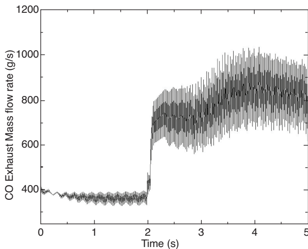
Figure 18 CO exhaust mass flow rate.
