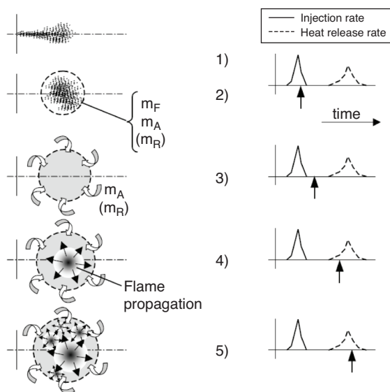
Figure 2 Evolution of the pre-mixed zone (from [1]).
